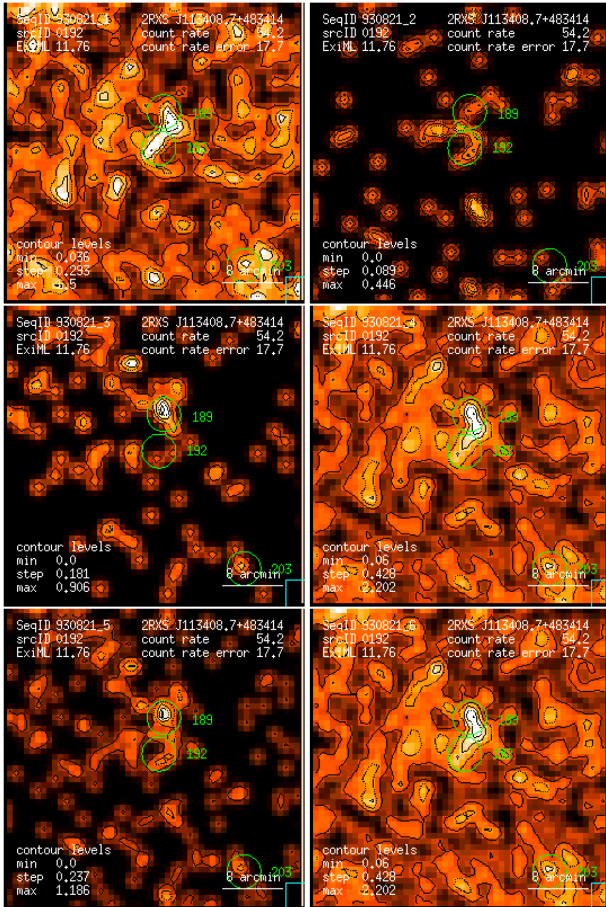
Figure 192: RASS 930821: detection 0192: band rate images, Gaussian filter: (1) PSPC channels 11 – 41, (2) 52 – 90, (3) 91 – 201, (4) 11 – 235, (5) 52 – 201, (6) 11 – 201. Broad band rates in counts/ks. Band rate contour levels in counts/ks/arcmin 2 .
