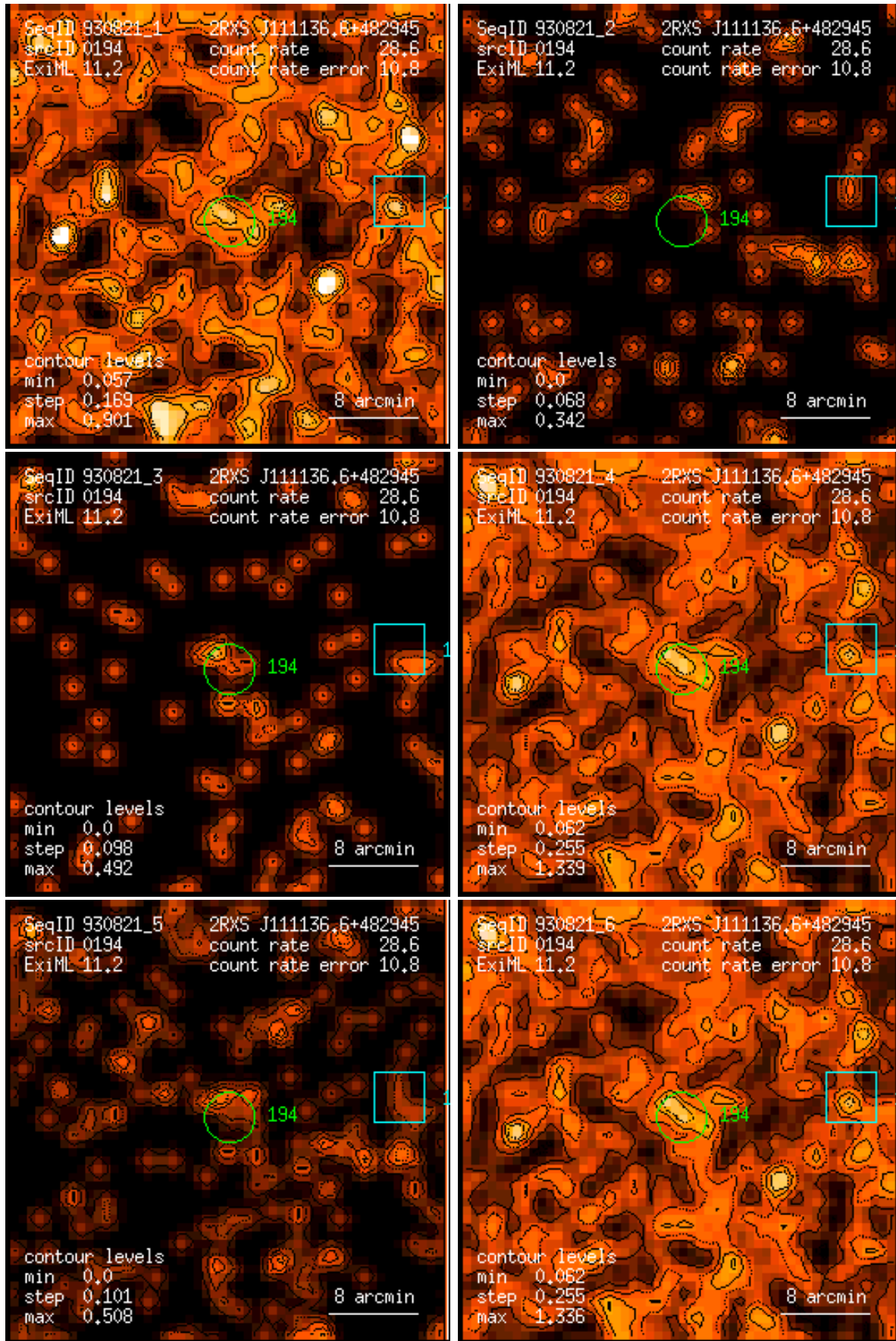
Figure 194: RASS 930821: detection 0194: band rate images, Gaussian filter: (1) PSPC channels 11 – 41, (2) 52 – 90, (3) 91 – 201, (4) 11 – 235, (5) 52 – 201, (6) 11 – 201. Broad band rates in counts/ks. Band rate contour levels in counts/ks/arcmin 2 .
