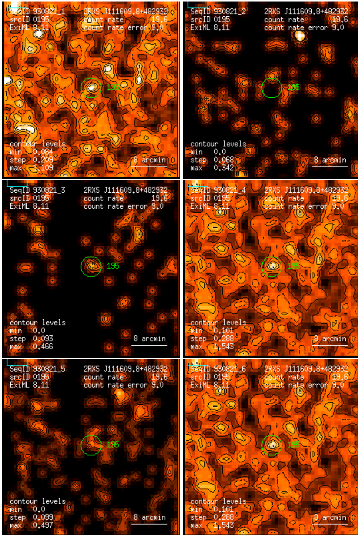
Figure 195: RASS 930821: detection 0195: band rate images, Gaussian filter: (1) PSPC channels 11 – 41, (2) 52 – 90, (3) 91 – 201, (4) 11 – 235, (5) 52 – 201, (6) 11 – 201. Broad band rates in counts/ks. Band rate contour levels in counts/ks/arcmin 2 .
