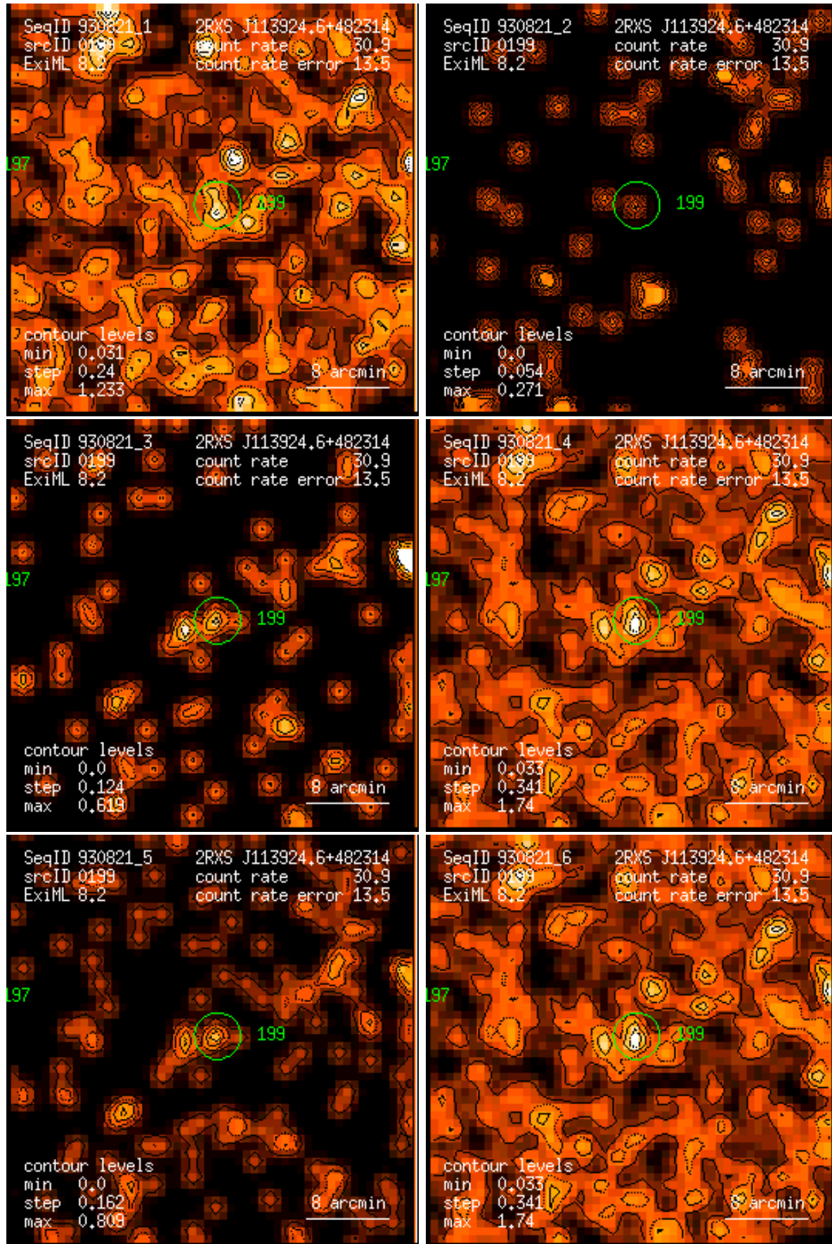
Figure 199: RASS 930821: detection 0199: band rate images, Gaussian filter: (1) PSPC channels 11 – 41, (2) 52 – 90, (3) 91 – 201, (4) 11 – 235, (5) 52 – 201, (6) 11 – 201. Broad band rates in counts/ks. Band rate contour levels in counts/ks/arcmin 2 .
