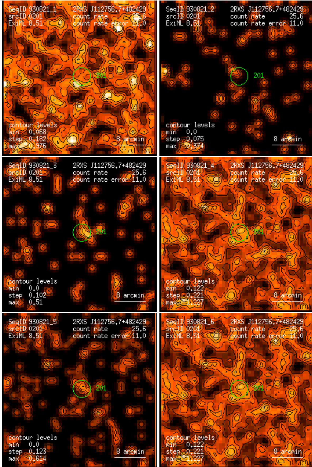
Figure 201: RASS 930821: detection 0201: band rate images, Gaussian filter: (1) PSPC channels 11 – 41, (2) 52 – 90, (3) 91 – 201, (4) 11 – 235, (5) 52 – 201, (6) 11 – 201. Broad band rates in counts/ks. Band rate contour levels in counts/ks/arcmin 2 .
