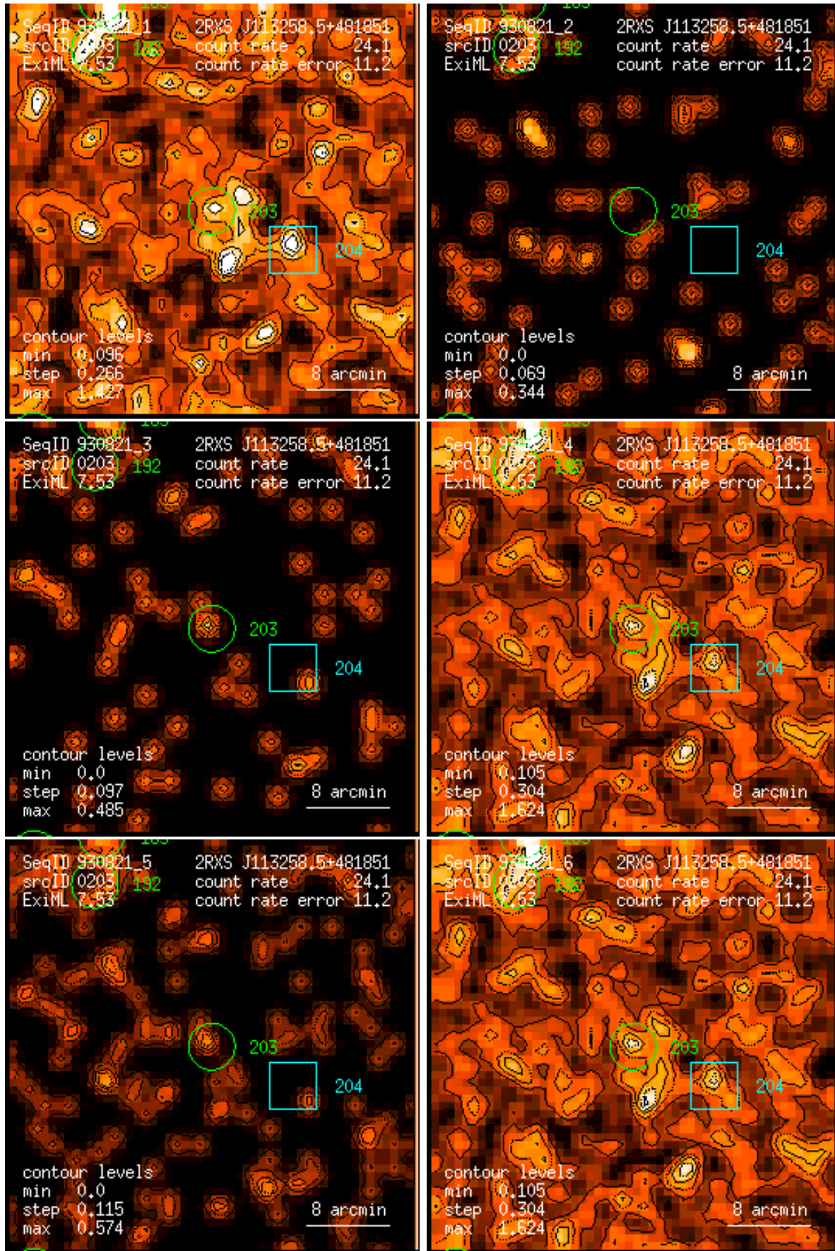
Figure 203: RASS 930821: detection 0203: band rate images, Gaussian filter: (1) PSPC channels 11 – 41, (2) 52 – 90, (3) 91 – 201, (4) 11 – 235, (5) 52 – 201, (6) 11 – 201. Broad band rates in counts/ks. Band rate contour levels in counts/ks/arcmin 2 .
