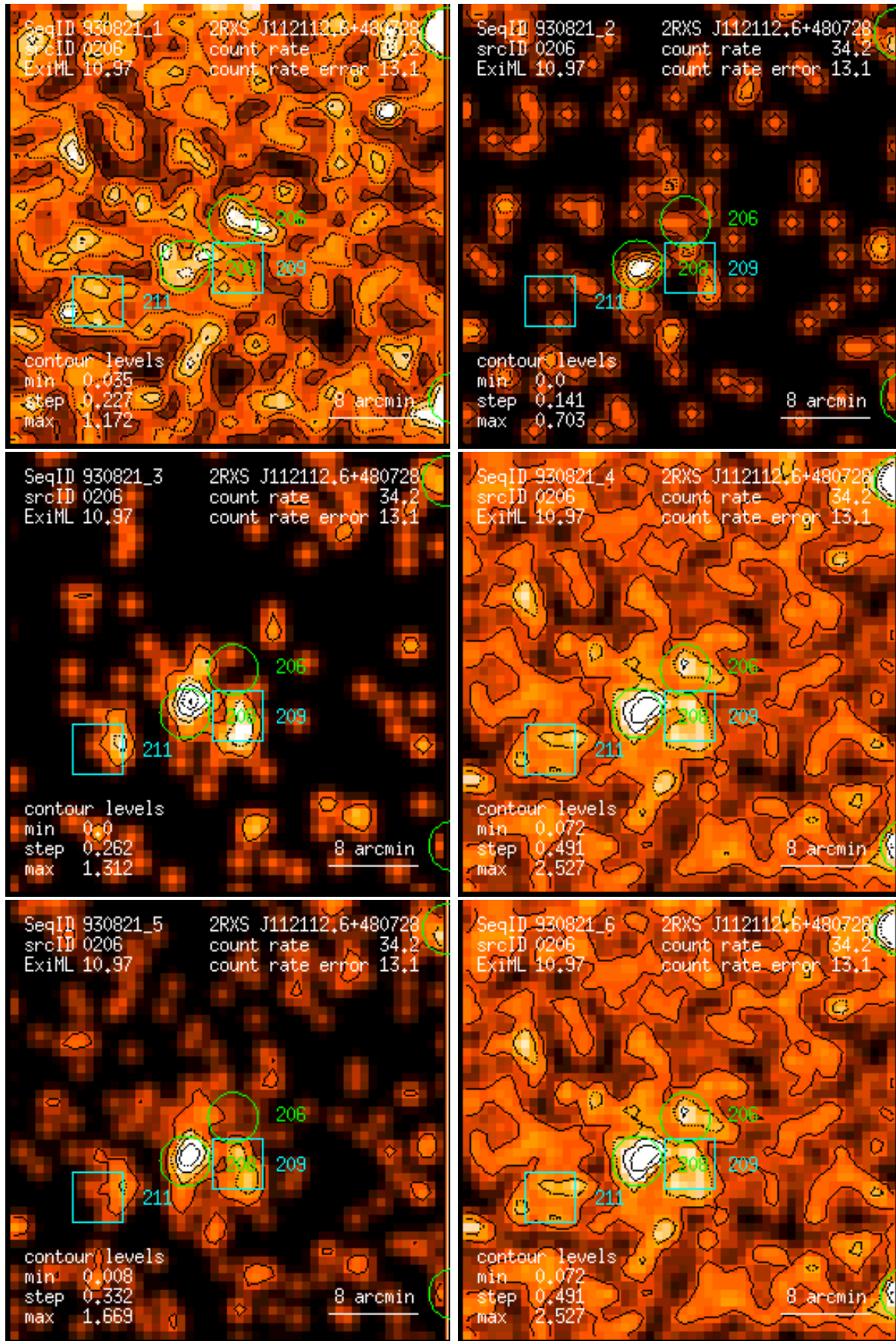
Figure 206: RASS 930821: detection 0206: band rate images, Gaussian filter: (1) PSPC channels 11 – 41, (2) 52 – 90, (3) 91 – 201, (4) 11 – 235, (5) 52 – 201, (6) 11 – 201. Broad band rates in counts/ks. Band rate contour levels in counts/ks/arcmin 2 .
