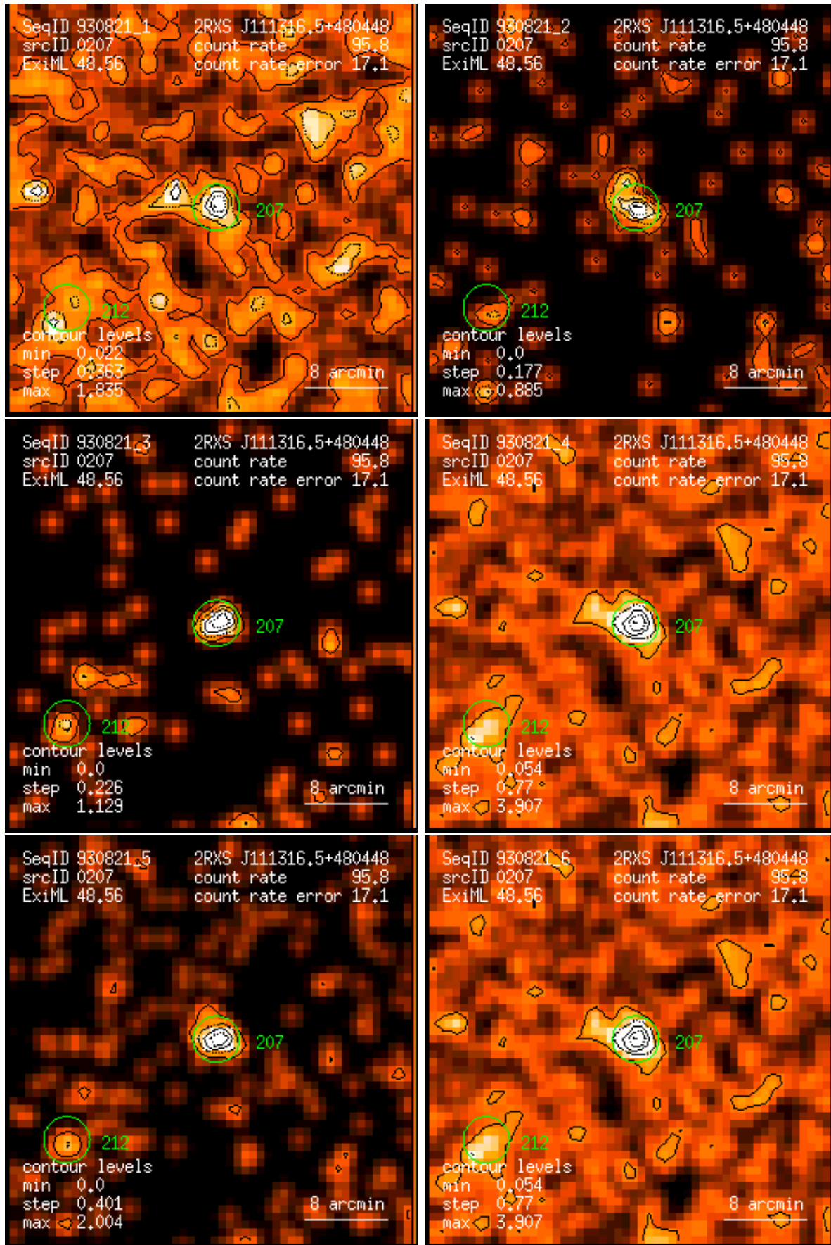
Figure 207: RASS 930821: detection 0207: band rate images, Gaussian filter: (1) PSPC channels 11 – 41, (2) 52 – 90, (3) 91 – 201, (4) 11 – 235, (5) 52 – 201, (6) 11 – 201. Broad band rates in counts/ks. Band rate contour levels in counts/ks/arcmin 2 .
