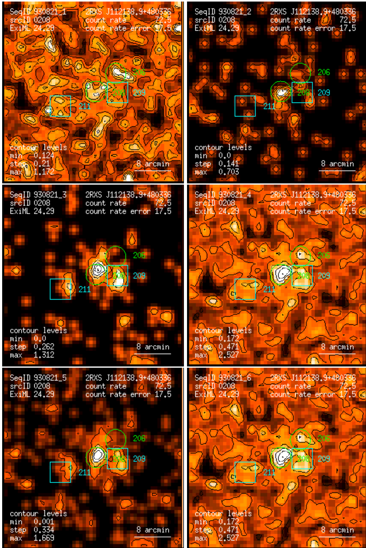
Figure 208: RASS 930821: detection 0208: band rate images, Gaussian filter: (1) PSPC channels 11 – 41, (2) 52 – 90, (3) 91 – 201, (4) 11 – 235, (5) 52 – 201, (6) 11 – 201. Broad band rates in counts/ks. Band rate contour levels in counts/ks/arcmin 2 .
