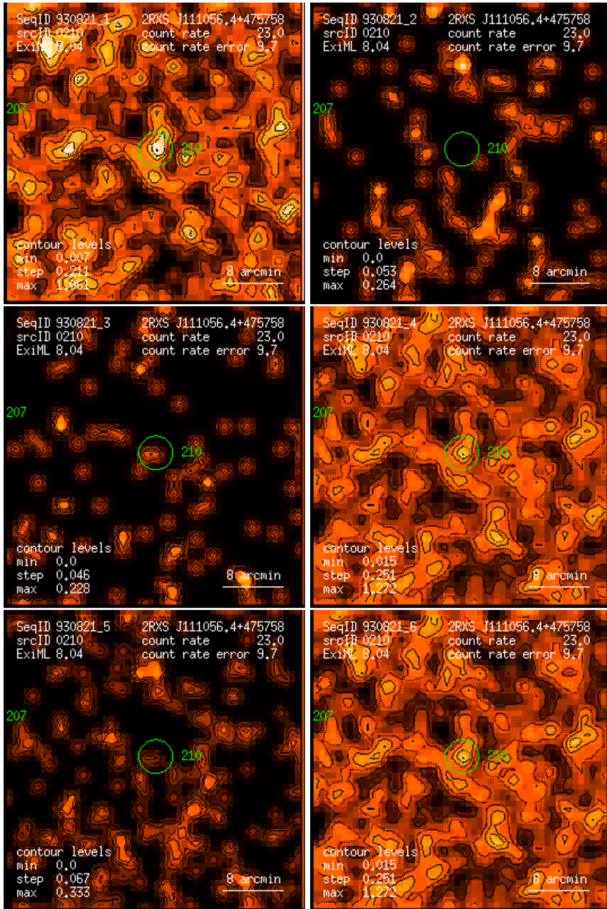
Figure 210: RASS 930821: detection 0210: band rate images, Gaussian filter: (1) PSPC channels 11 – 41, (2) 52 – 90, (3) 91 – 201, (4) 11 – 235, (5) 52 – 201, (6) 11 – 201. Broad band rates in counts/ks. Band rate contour levels in counts/ks/arcmin 2 .
