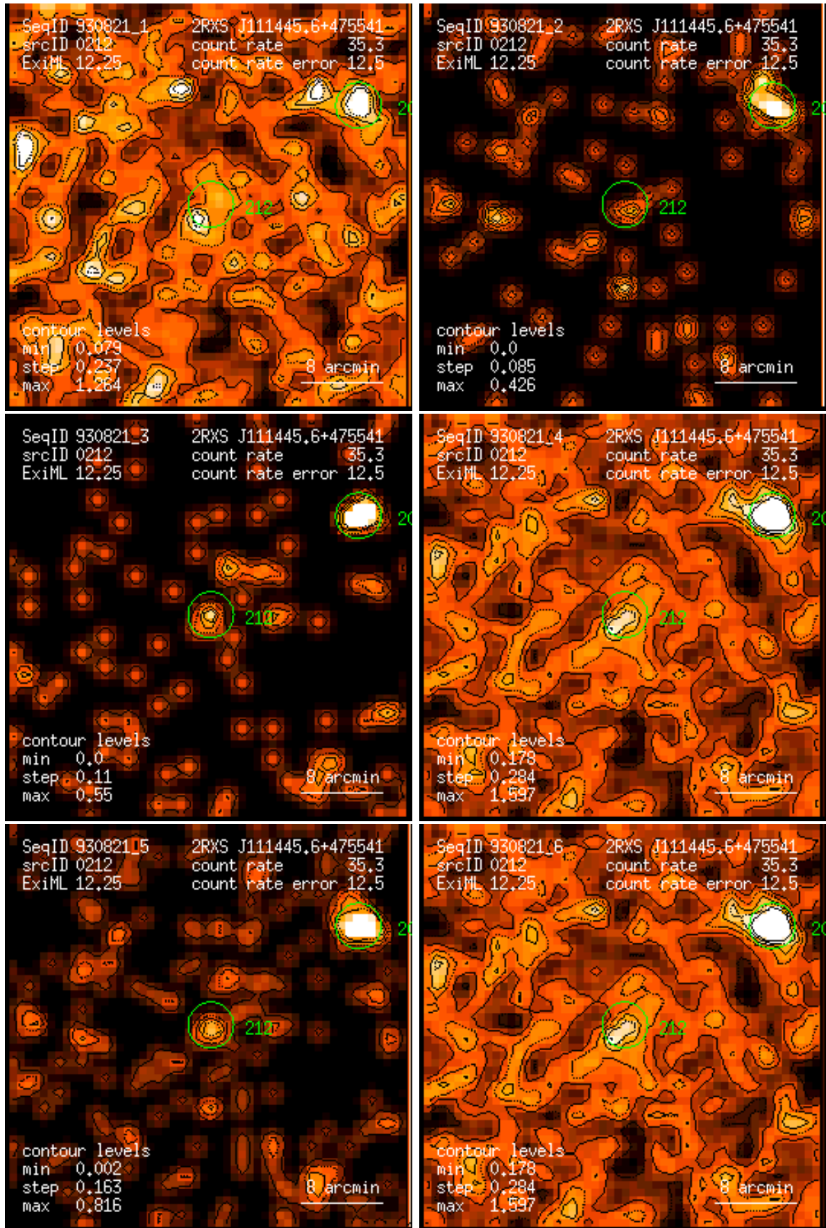
Figure 212: RASS 930821: detection 0212: band rate images, Gaussian filter: (1) PSPC channels 11 – 41, (2) 52 – 90, (3) 91 – 201, (4) 11 – 235, (5) 52 – 201, (6) 11 – 201. Broad band rates in counts/ks. Band rate contour levels in counts/ks/arcmin 2 .
