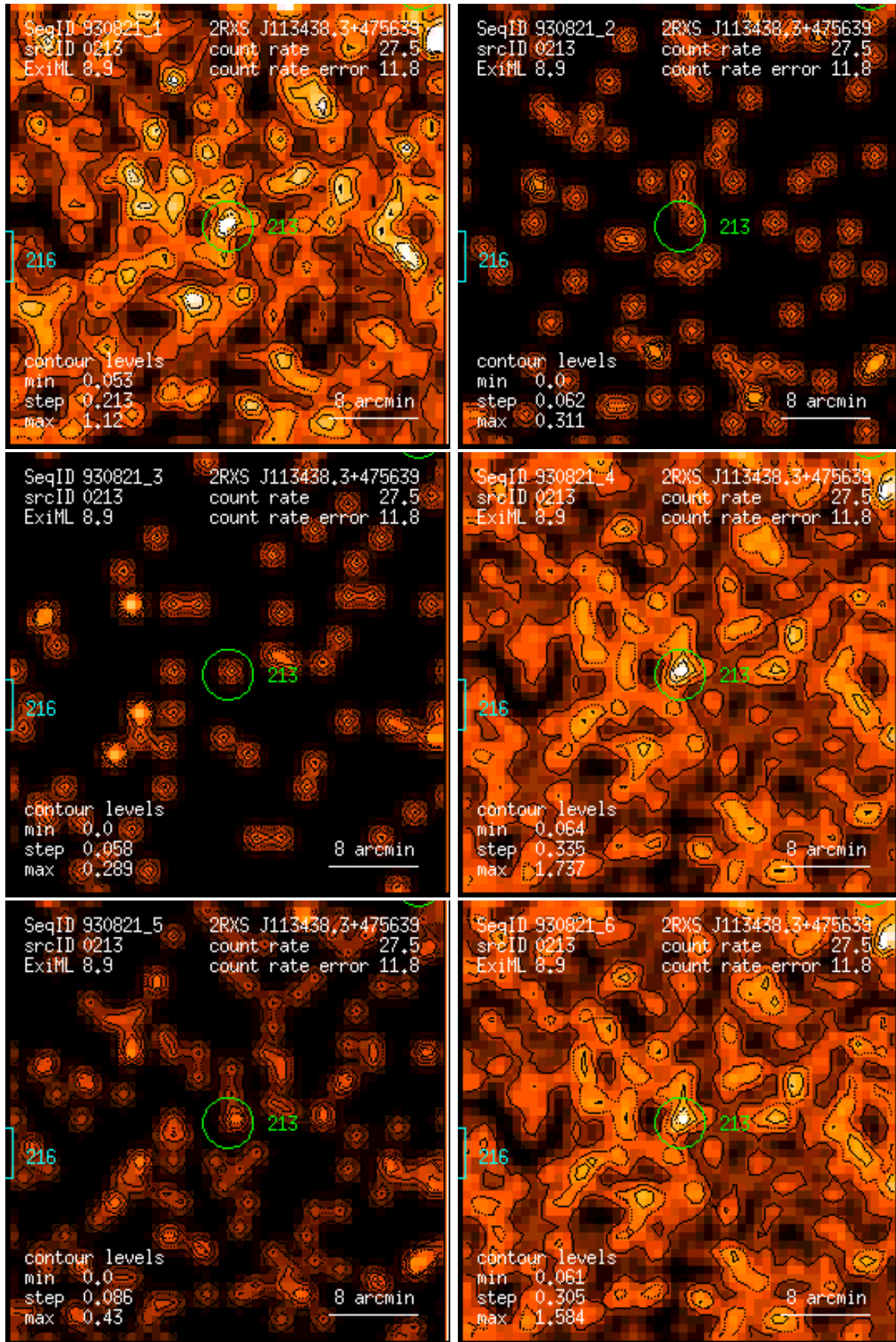
Figure 213: RASS 930821: detection 0213: band rate images, Gaussian filter: (1) PSPC channels 11 – 41, (2) 52 – 90, (3) 91 – 201, (4) 11 – 235, (5) 52 – 201, (6) 11 – 201. Broad band rates in counts/ks. Band rate contour levels in counts/ks/arcmin 2 .
