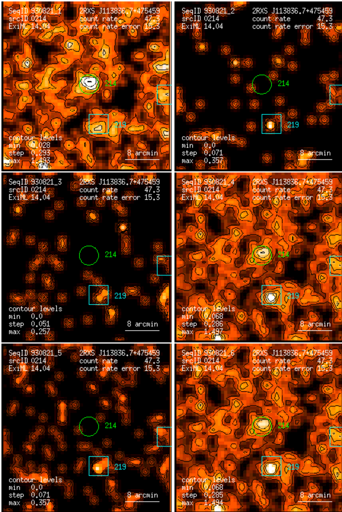
Figure 214: RASS 930821: detection 0214: band rate images, Gaussian filter: (1) PSPC channels 11 – 41, (2) 52 – 90, (3) 91 – 201, (4) 11 – 235, (5) 52 – 201, (6) 11 – 201. Broad band rates in counts/ks. Band rate contour levels in counts/ks/arcmin 2 .
