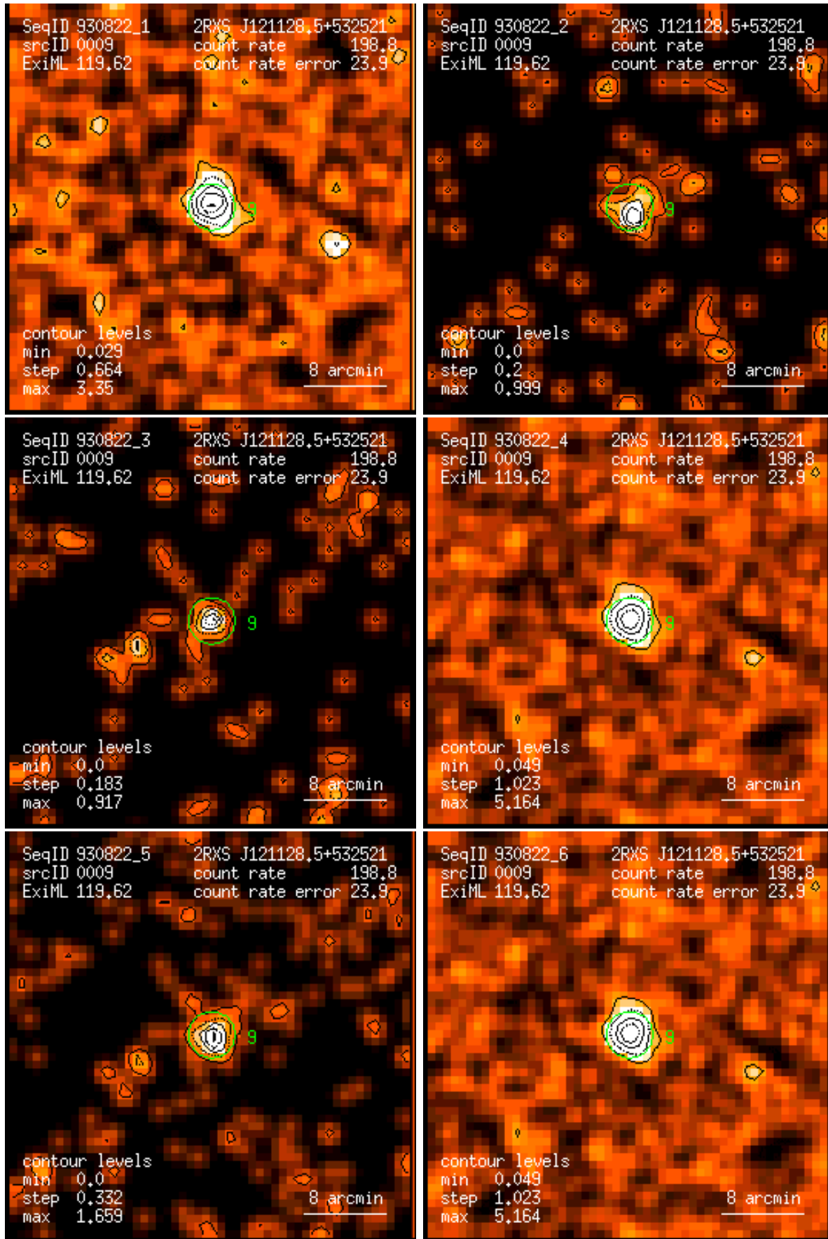
Figure 9: RASS 930822: detection 0009: band rate images, Gaussian filter: (1) PSPC channels 11 – 41, (2) 52 – 90, (3) 91 – 201, (4) 11 – 235, (5) 52 – 201, (6) 11 – 201. Broad band rates in counts/ks. Band rate contour levels in counts/ks/arcmin 2 .
