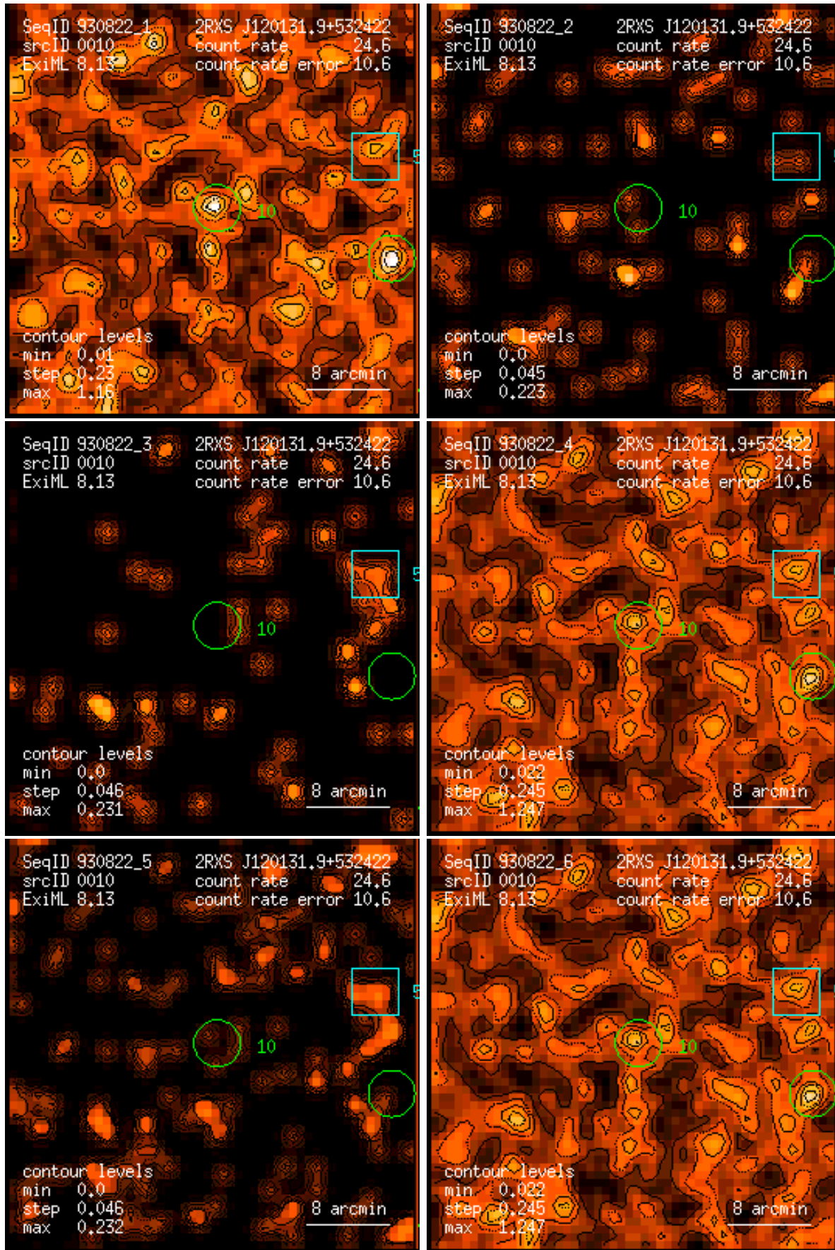
Figure 10: RASS 930822: detection 0010: band rate images, Gaussian filter: (1) PSPC channels 11 – 41, (2) 52 – 90, (3) 91 – 201, (4) 11 – 235, (5) 52 – 201, (6) 11 – 201. Broad band rates in counts/ks. Band rate contour levels in counts/ks/arcmin 2 .
