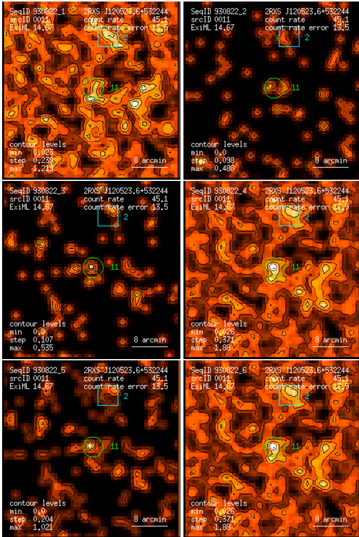
Figure 11: RASS 930822: detection 0011: band rate images, Gaussian filter: (1) PSPC channels 11 – 41, (2) 52 – 90, (3) 91 – 201, (4) 11 – 235, (5) 52 – 201, (6) 11 – 201. Broad band rates in counts/ks. Band rate contour levels in counts/ks/arcmin 2 .
