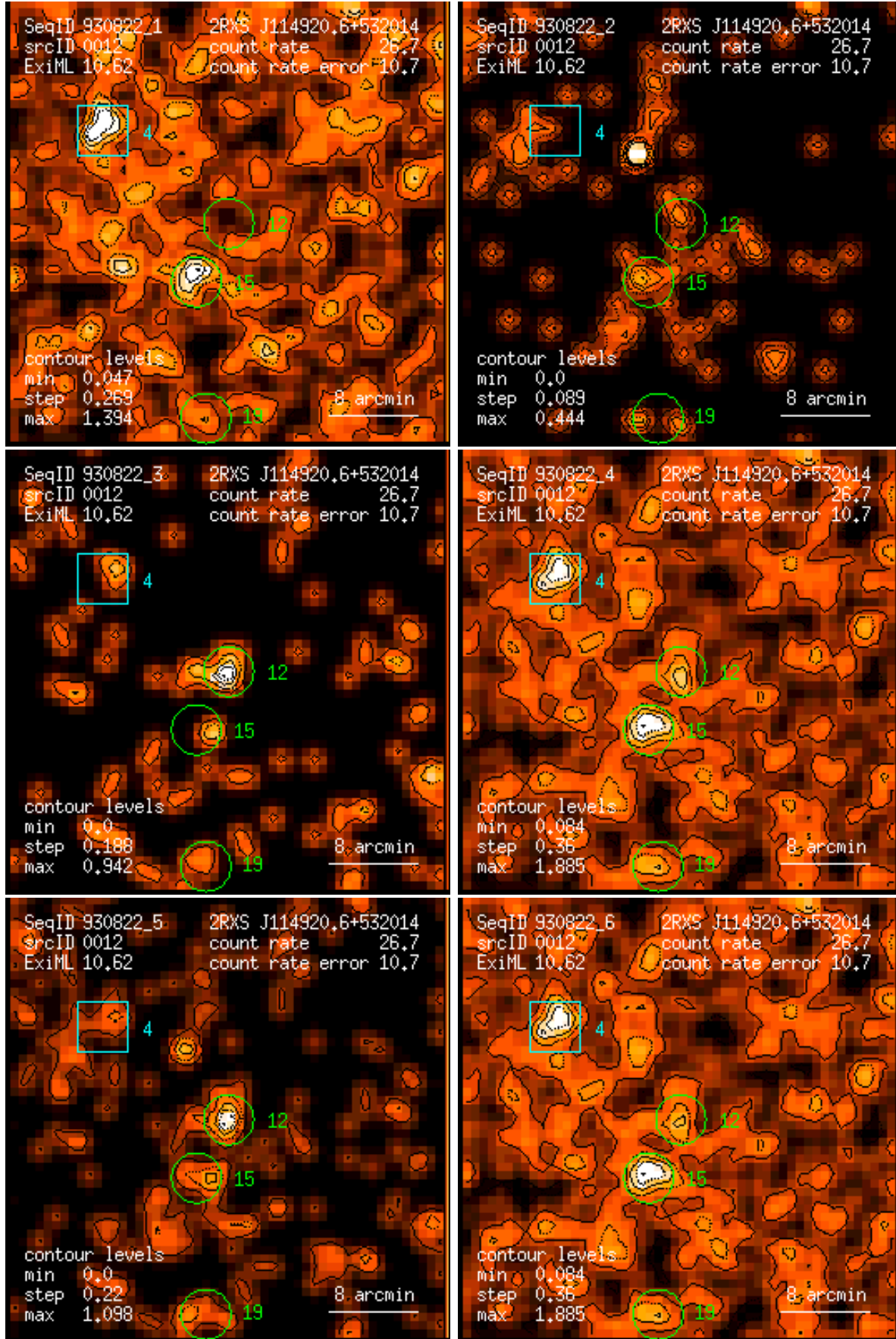
Figure 12: RASS 930822: detection 0012: band rate images, Gaussian filter: (1) PSPC channels 11 – 41, (2) 52 – 90, (3) 91 – 201, (4) 11 – 235, (5) 52 – 201, (6) 11 – 201. Broad band rates in counts/ks. Band rate contour levels in counts/ks/arcmin 2 .
