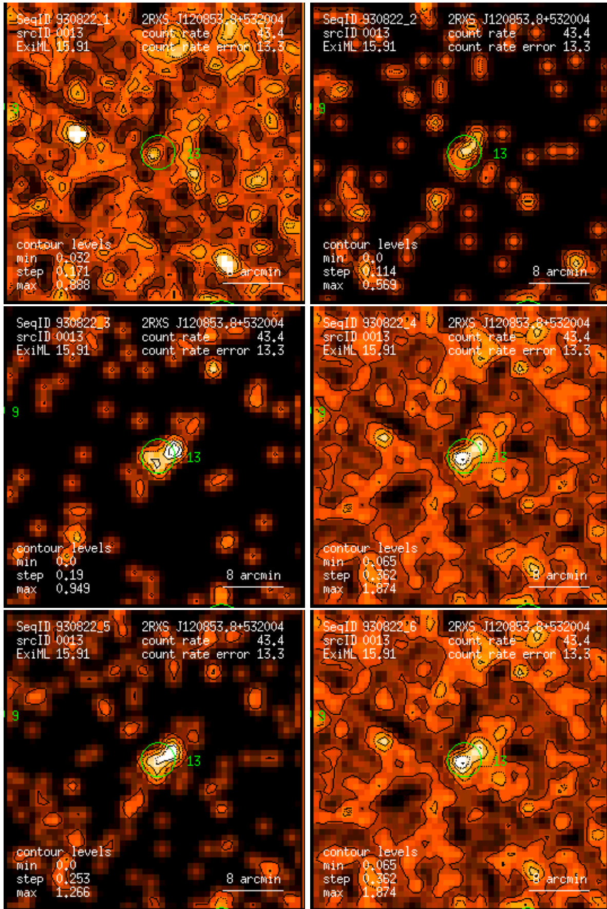
Figure 13: RASS 930822: detection 0013: band rate images, Gaussian filter: (1) PSPC channels 11 – 41, (2) 52 – 90, (3) 91 – 201, (4) 11 – 235, (5) 52 – 201, (6) 11 – 201. Broad band rates in counts/ks. Band rate contour levels in counts/ks/arcmin 2 .
