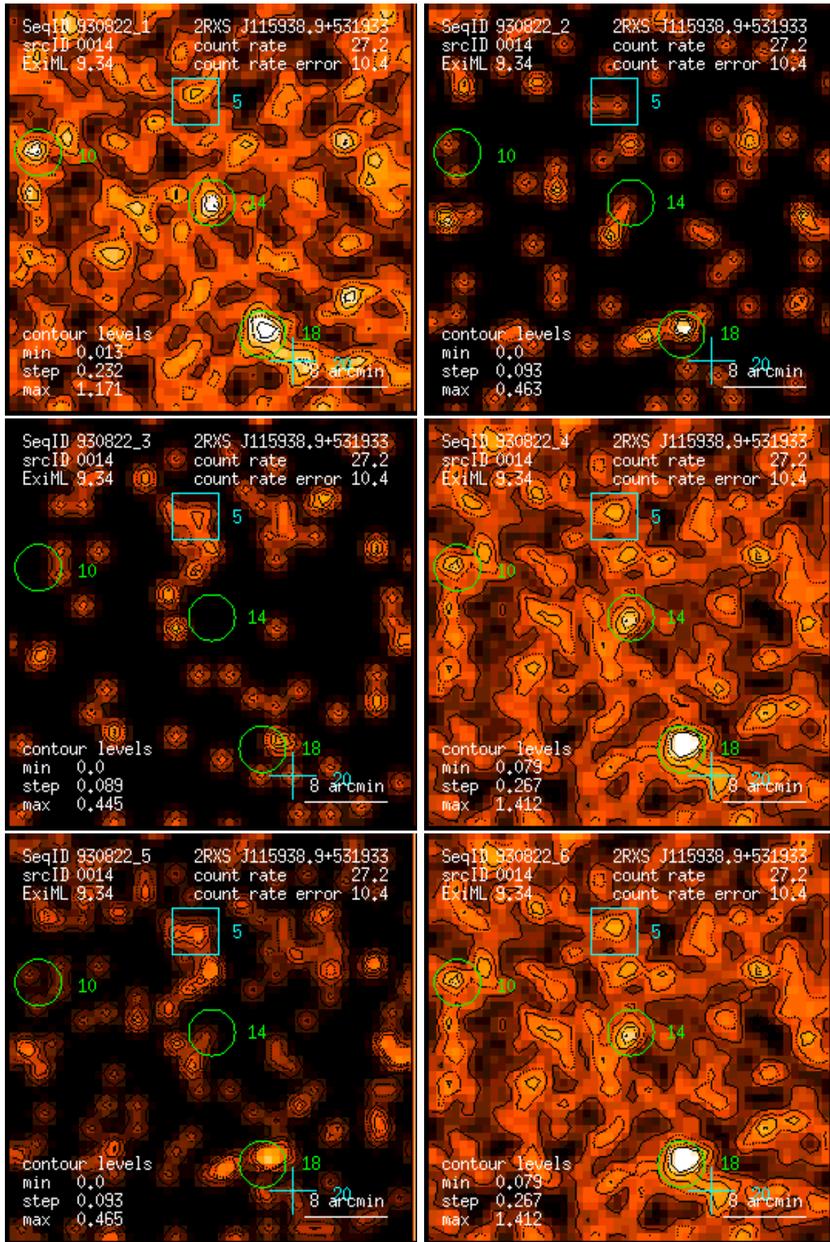
Figure 14: RASS 930822: detection 0014: band rate images, Gaussian filter: (1) PSPC channels 11 – 41, (2) 52 – 90, (3) 91 – 201, (4) 11 – 235, (5) 52 – 201, (6) 11 – 201. Broad band rates in counts/ks. Band rate contour levels in counts/ks/arcmin 2 .
