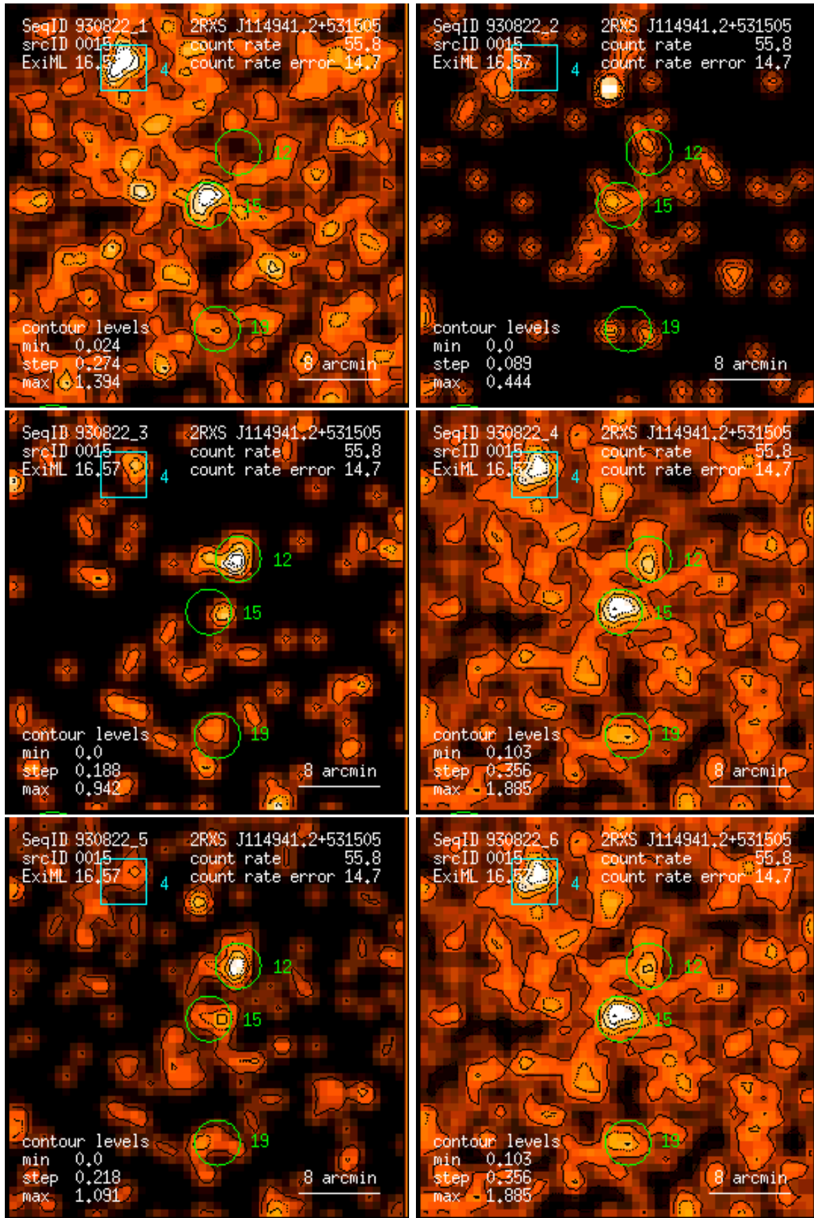
Figure 15: RASS 930822: detection 0015: band rate images, Gaussian filter: (1) PSPC channels 11 – 41, (2) 52 – 90, (3) 91 – 201, (4) 11 – 235, (5) 52 – 201, (6) 11 – 201. Broad band rates in counts/ks. Band rate contour levels in counts/ks/arcmin 2 .
