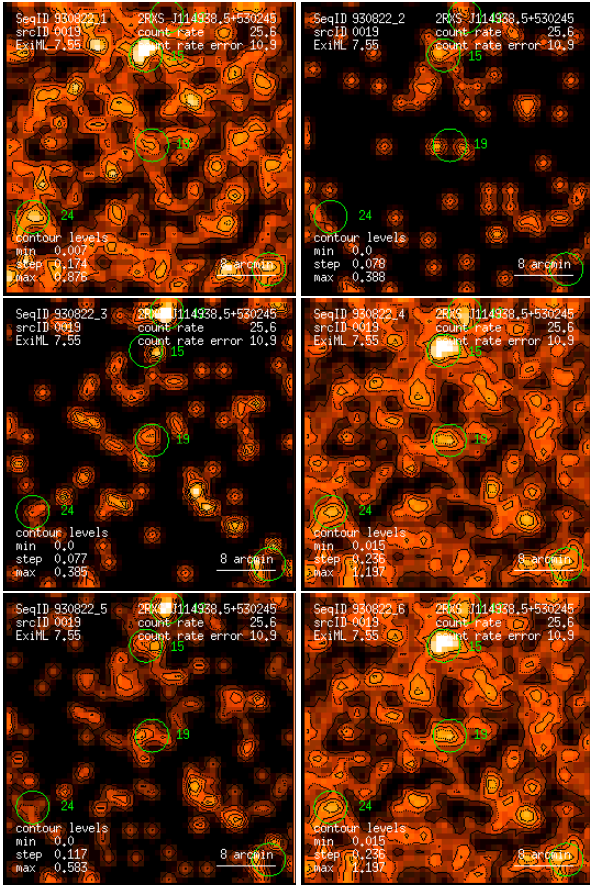
Figure 19: RASS 930822: detection 0019: band rate images, Gaussian filter: (1) PSPC channels 11 – 41, (2) 52 – 90, (3) 91 – 201, (4) 11 – 235, (5) 52 – 201, (6) 11 – 201. Broad band rates in counts/ks. Band rate contour levels in counts/ks/arcmin 2 .
