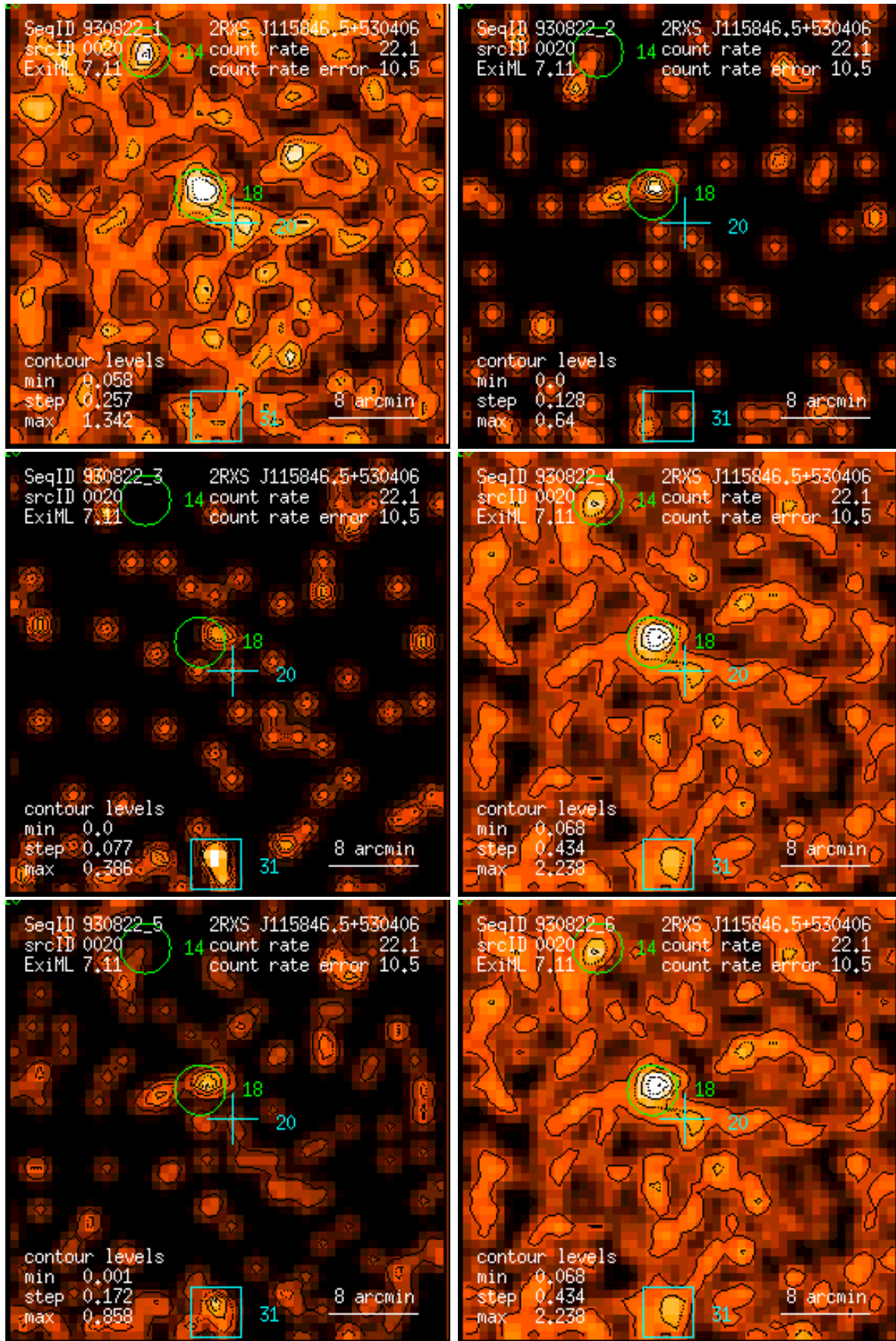
Figure 20: RASS 930822: detection 0020: band rate images, Gaussian filter: (1) PSPC channels 11 – 41, (2) 52 – 90, (3) 91 – 201, (4) 11 – 235, (5) 52 – 201, (6) 11 – 201. Broad band rates in counts/ks. Band rate contour levels in counts/ks/arcmin 2 .
