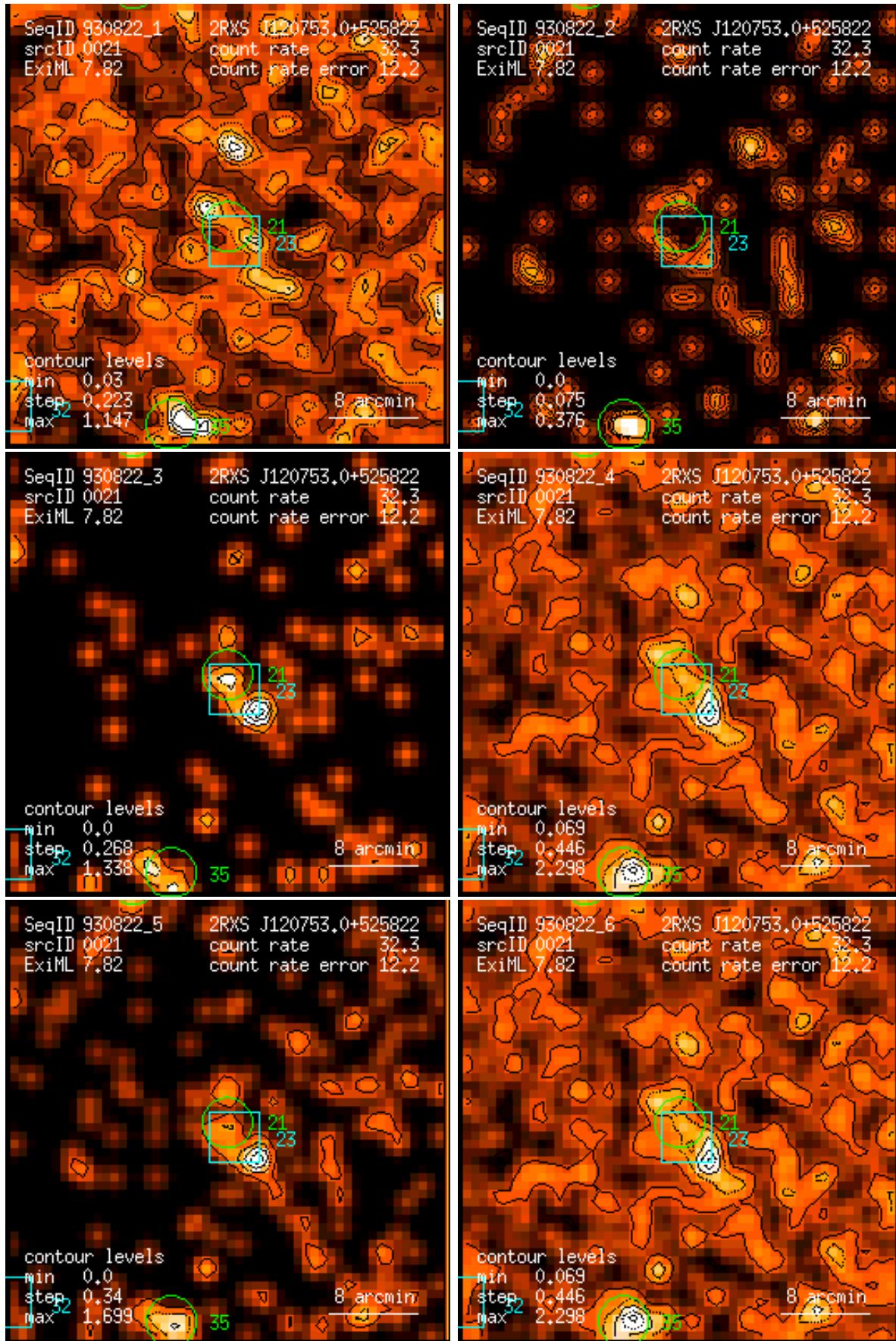
Figure 21: RASS 930822: detection 0021: band rate images, Gaussian filter: (1) PSPC channels 11 – 41, (2) 52 – 90, (3) 91 – 201, (4) 11 – 235, (5) 52 – 201, (6) 11 – 201. Broad band rates in counts/ks. Band rate contour levels in counts/ks/arcmin 2 .
