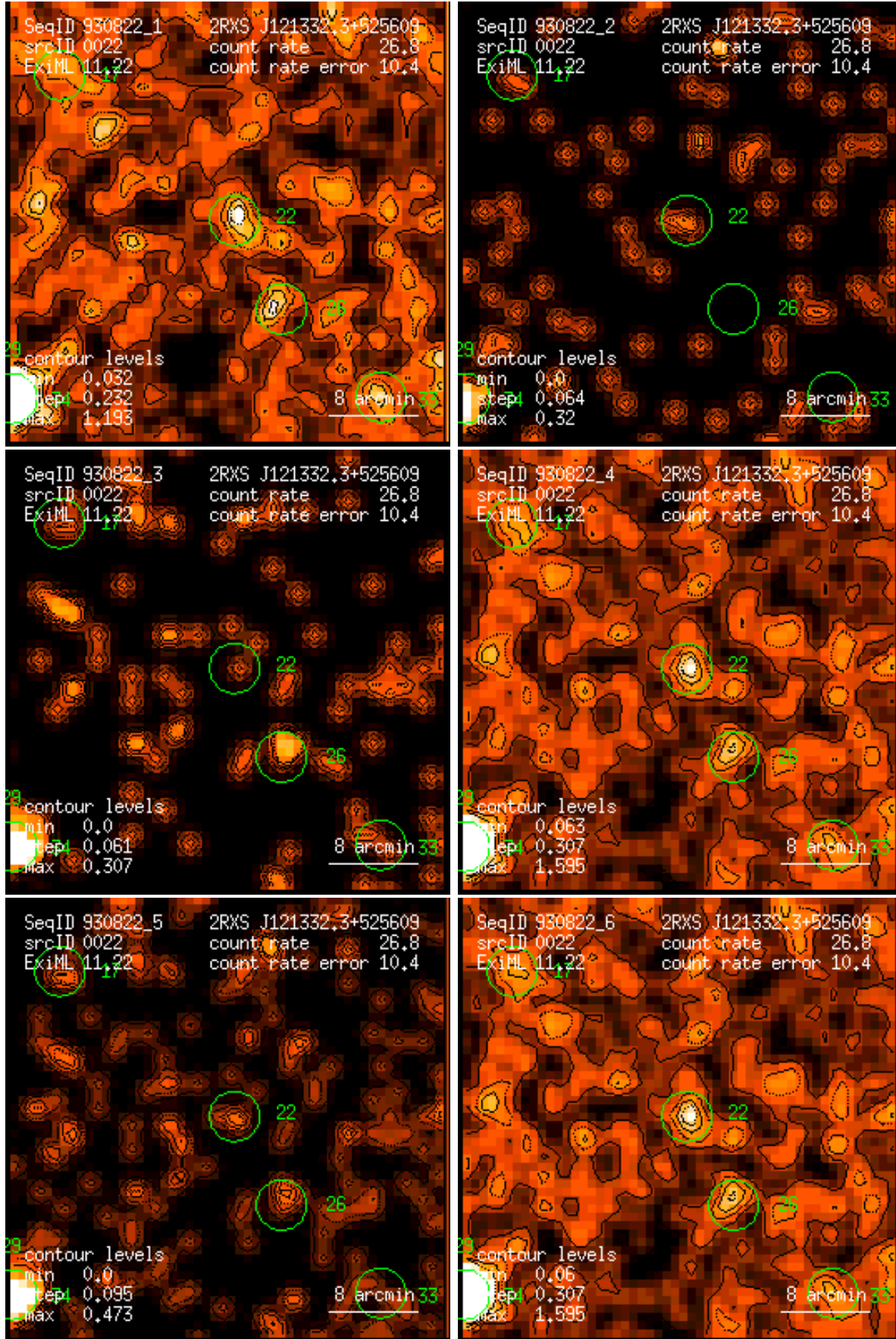
Figure 22: RASS 930822: detection 0022: band rate images, Gaussian filter: (1) PSPC channels 11 – 41, (2) 52 – 90, (3) 91 – 201, (4) 11 – 235, (5) 52 – 201, (6) 11 – 201. Broad band rates in counts/ks. Band rate contour levels in counts/ks/arcmin 2 .
