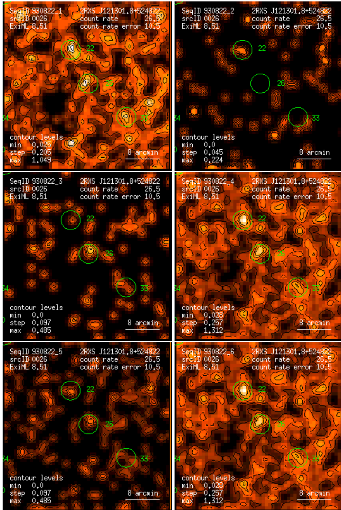
Figure 26: RASS 930822: detection 0026: band rate images, Gaussian filter: (1) PSPC channels 11 – 41, (2) 52 – 90, (3) 91 – 201, (4) 11 – 235, (5) 52 – 201, (6) 11 – 201. Broad band rates in counts/ks. Band rate contour levels in counts/ks/arcmin 2 .
