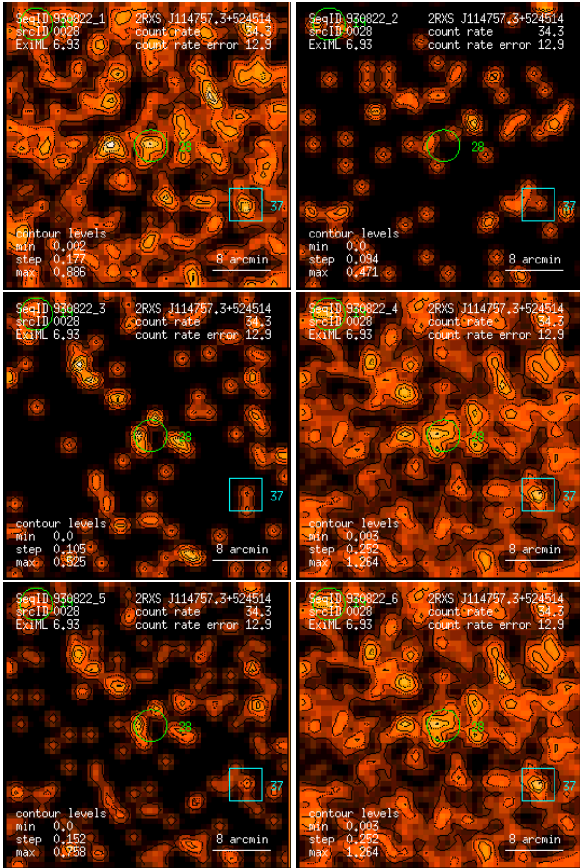
Figure 28: RASS 930822: detection 0028: band rate images, Gaussian filter: (1) PSPC channels 11 – 41, (2) 52 – 90, (3) 91 – 201, (4) 11 – 235, (5) 52 – 201, (6) 11 – 201. Broad band rates in counts/ks. Band rate contour levels in counts/ks/arcmin 2 .
