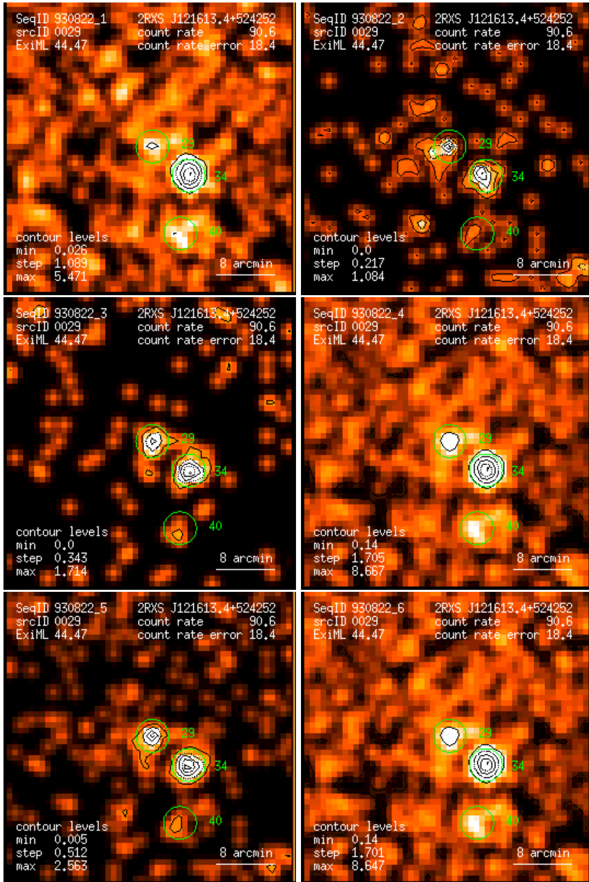
Figure 29: RASS 930822: detection 0029: band rate images, Gaussian filter: (1) PSPC channels 11 – 41, (2) 52 – 90, (3) 91 – 201, (4) 11 – 235, (5) 52 – 201, (6) 11 – 201. Broad band rates in counts/ks. Band rate contour levels in counts/ks/arcmin 2 .
