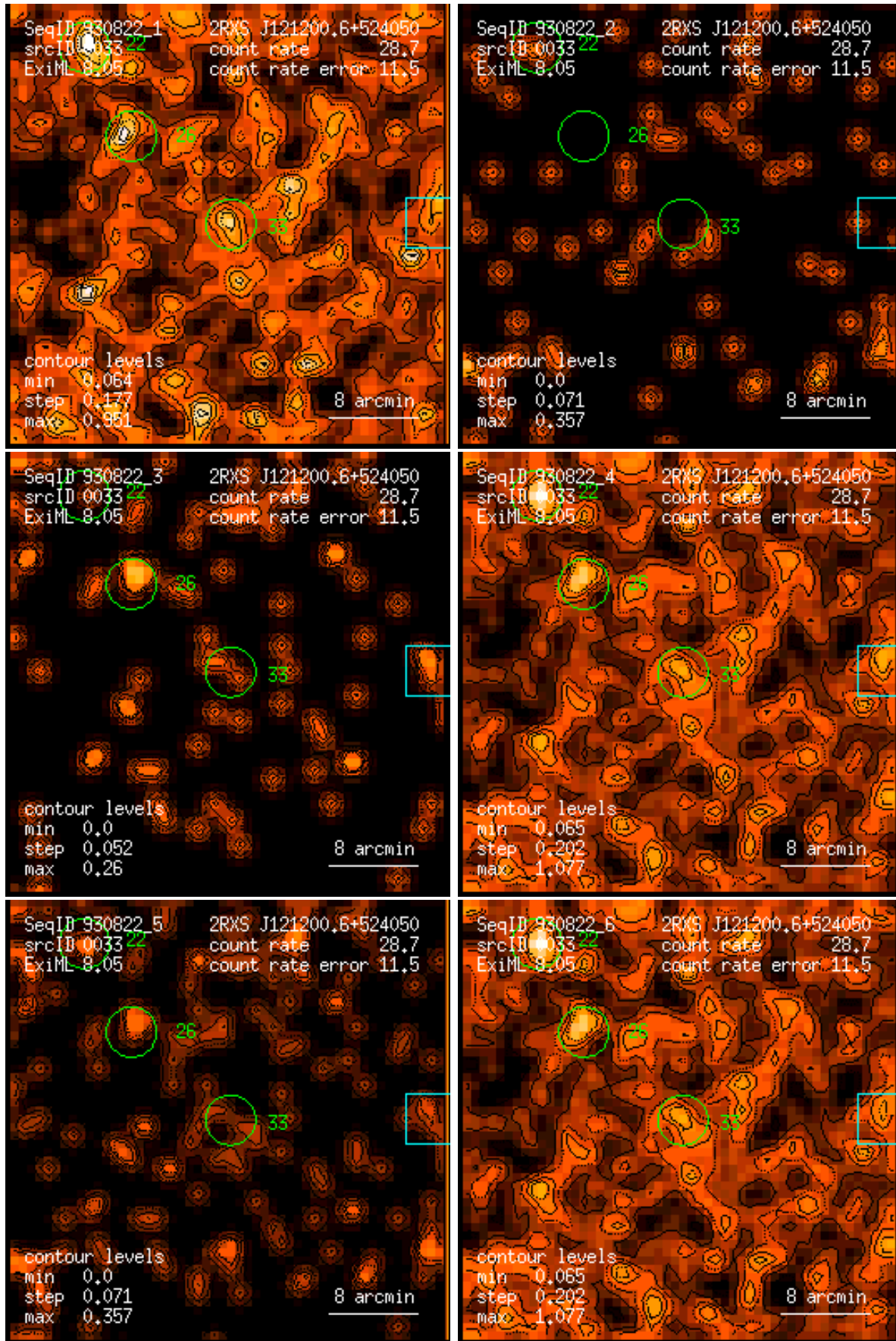
Figure 33: RASS 930822: detection 0033: band rate images, Gaussian filter: (1) PSPC channels 11 – 41, (2) 52 – 90, (3) 91 – 201, (4) 11 – 235, (5) 52 – 201, (6) 11 – 201. Broad band rates in counts/ks. Band rate contour levels in counts/ks/arcmin 2 .
