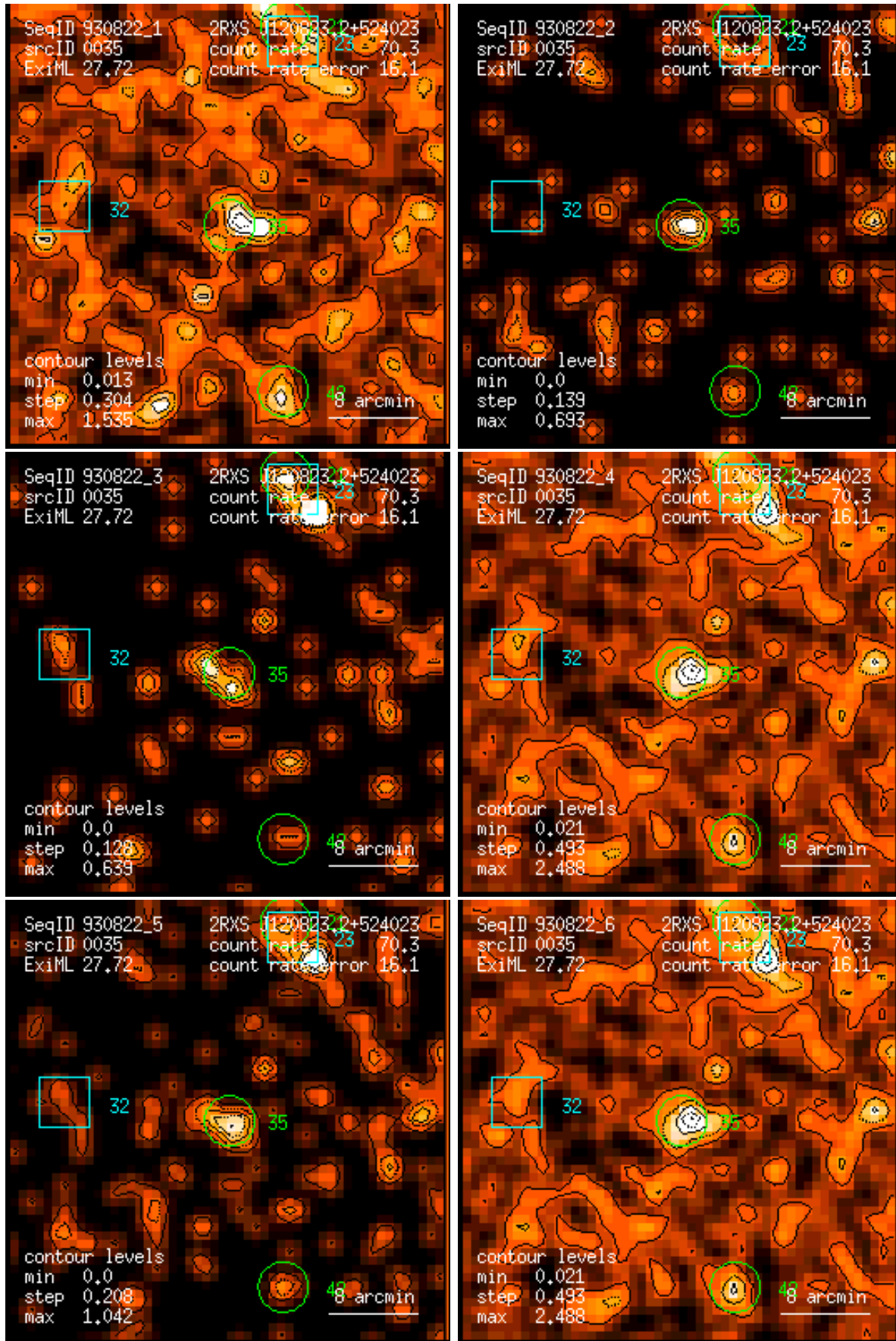
Figure 35: RASS 930822: detection 0035: band rate images, Gaussian filter: (1) PSPC channels 11 – 41, (2) 52 – 90, (3) 91 – 201, (4) 11 – 235, (5) 52 – 201, (6) 11 – 201. Broad band rates in counts/ks. Band rate contour levels in counts/ks/arcmin 2 .
