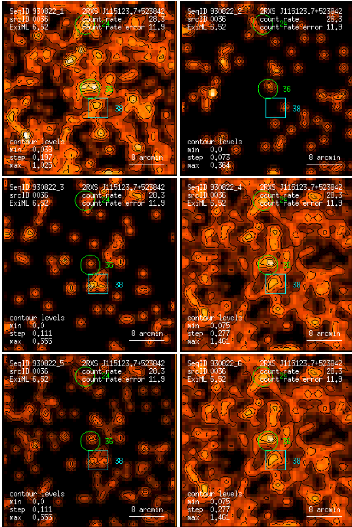
Figure 36: RASS 930822: detection 0036: band rate images, Gaussian filter: (1) PSPC channels 11 – 41, (2) 52 – 90, (3) 91 – 201, (4) 11 – 235, (5) 52 – 201, (6) 11 – 201. Broad band rates in counts/ks. Band rate contour levels in counts/ks/arcmin 2 .
