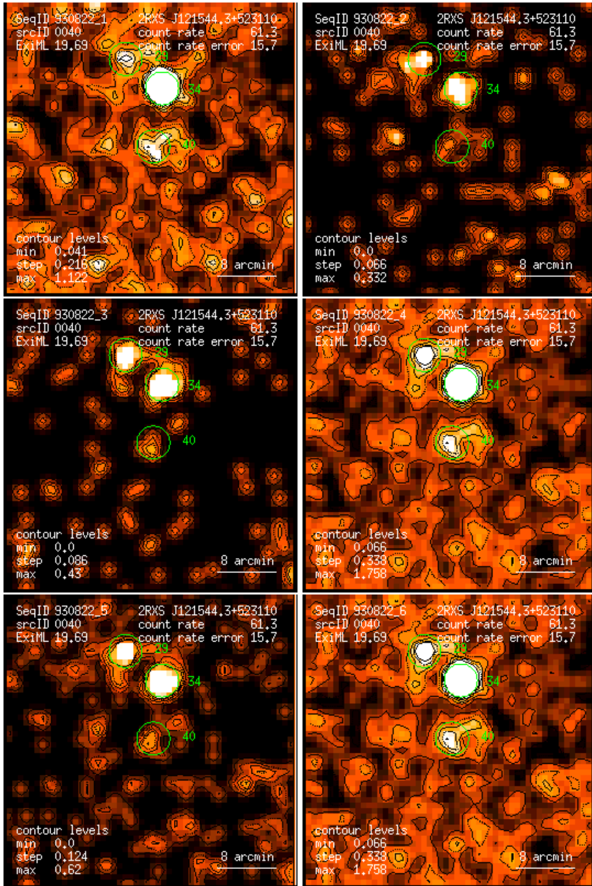
Figure 40: RASS 930822: detection 0040: band rate images, Gaussian filter: (1) PSPC channels 11 – 41, (2) 52 – 90, (3) 91 – 201, (4) 11 – 235, (5) 52 – 201, (6) 11 – 201. Broad band rates in counts/ks. Band rate contour levels in counts/ks/arcmin 2 .
