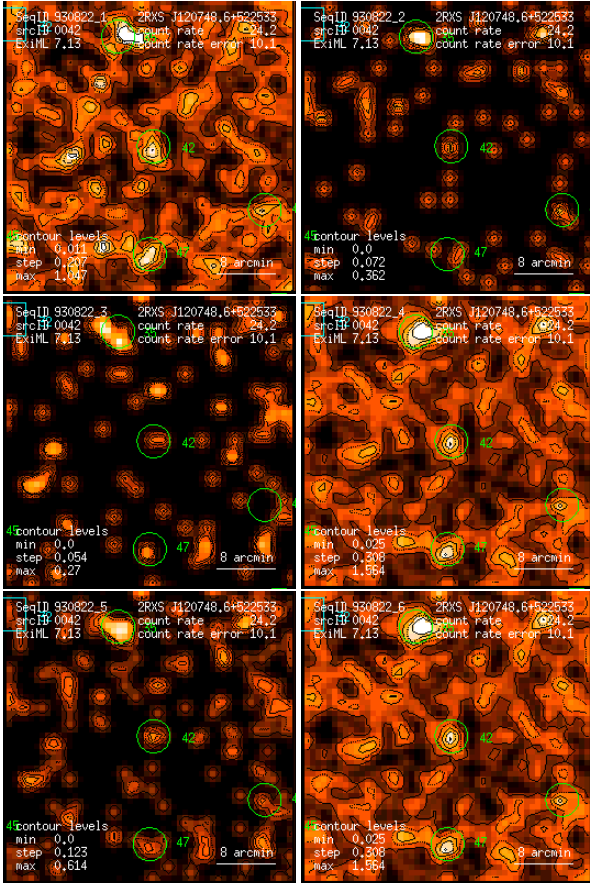
Figure 42: RASS 930822: detection 0042: band rate images, Gaussian filter: (1) PSPC channels 11 – 41, (2) 52 – 90, (3) 91 – 201, (4) 11 – 235, (5) 52 – 201, (6) 11 – 201. Broad band rates in counts/ks. Band rate contour levels in counts/ks/arcmin 2 .
