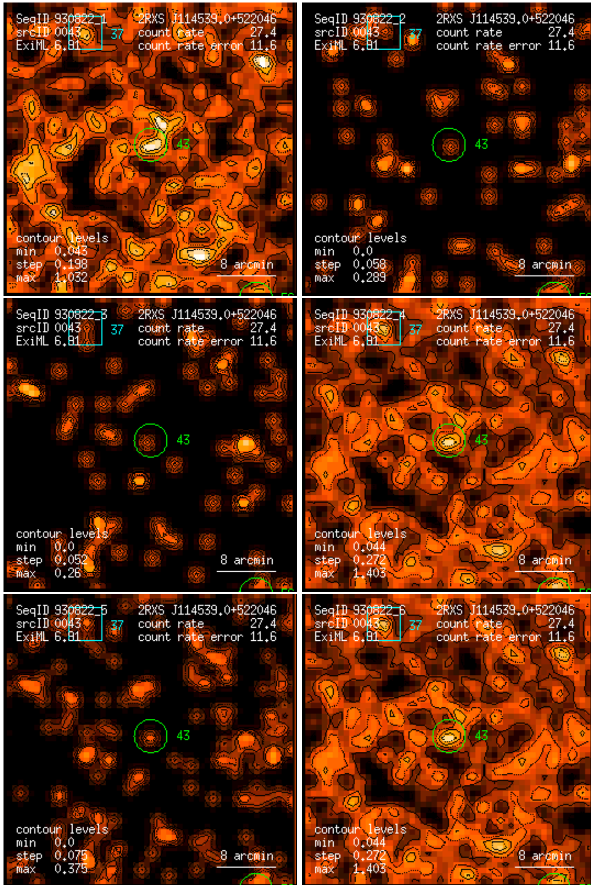
Figure 43: RASS 930822: detection 0043: band rate images, Gaussian filter: (1) PSPC channels 11 – 41, (2) 52 – 90, (3) 91 – 201, (4) 11 – 235, (5) 52 – 201, (6) 11 – 201. Broad band rates in counts/ks. Band rate contour levels in counts/ks/arcmin 2 .
