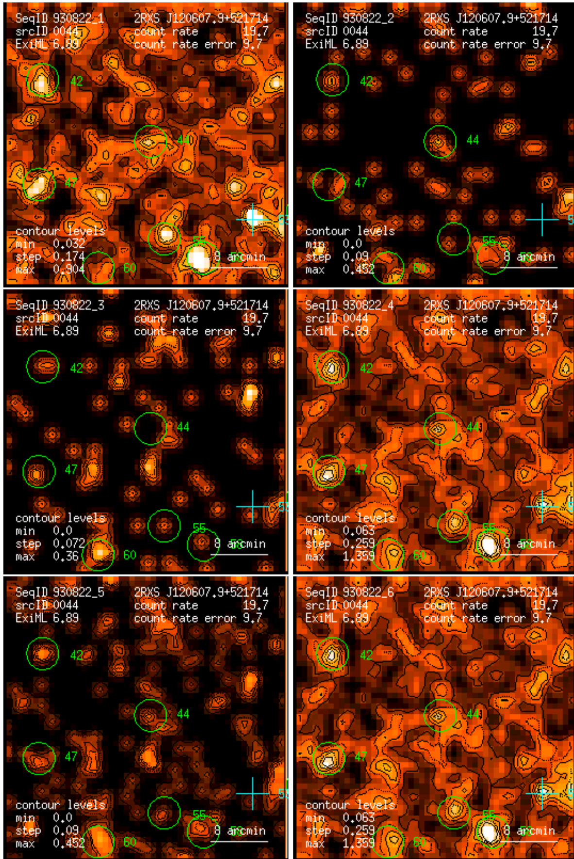
Figure 44: RASS 930822: detection 0044: band rate images, Gaussian filter: (1) PSPC channels 11 – 41, (2) 52 – 90, (3) 91 – 201, (4) 11 – 235, (5) 52 – 201, (6) 11 – 201. Broad band rates in counts/ks. Band rate contour levels in counts/ks/arcmin 2 .
