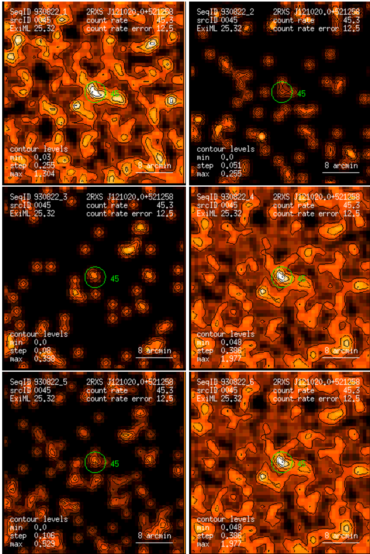
Figure 45: RASS 930822: detection 0045: band rate images, Gaussian filter: (1) PSPC channels 11 – 41, (2) 52 – 90, (3) 91 – 201, (4) 11 – 235, (5) 52 – 201, (6) 11 – 201. Broad band rates in counts/ks. Band rate contour levels in counts/ks/arcmin 2 .
