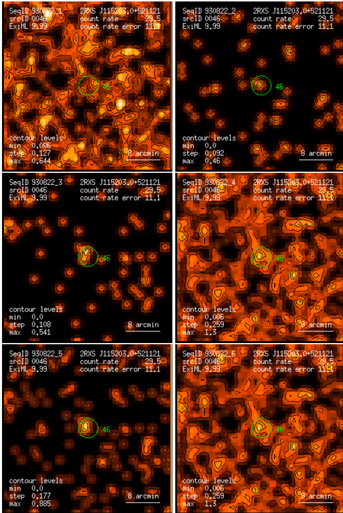
Figure 46: RASS 930822: detection 0046: band rate images, Gaussian filter: (1) PSPC channels 11 – 41, (2) 52 – 90, (3) 91 – 201, (4) 11 – 235, (5) 52 – 201, (6) 11 – 201. Broad band rates in counts/ks. Band rate contour levels in counts/ks/arcmin 2 .
