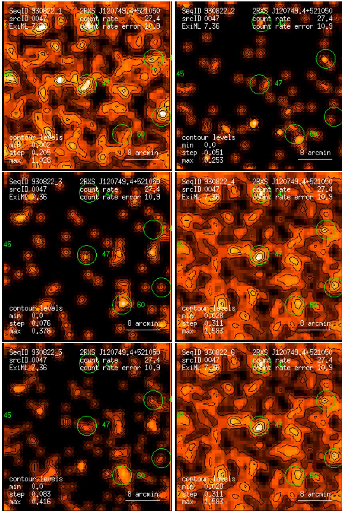
Figure 47: RASS 930822: detection 0047: band rate images, Gaussian filter: (1) PSPC channels 11 – 41, (2) 52 – 90, (3) 91 – 201, (4) 11 – 235, (5) 52 – 201, (6) 11 – 201. Broad band rates in counts/ks. Band rate contour levels in counts/ks/arcmin 2 .
