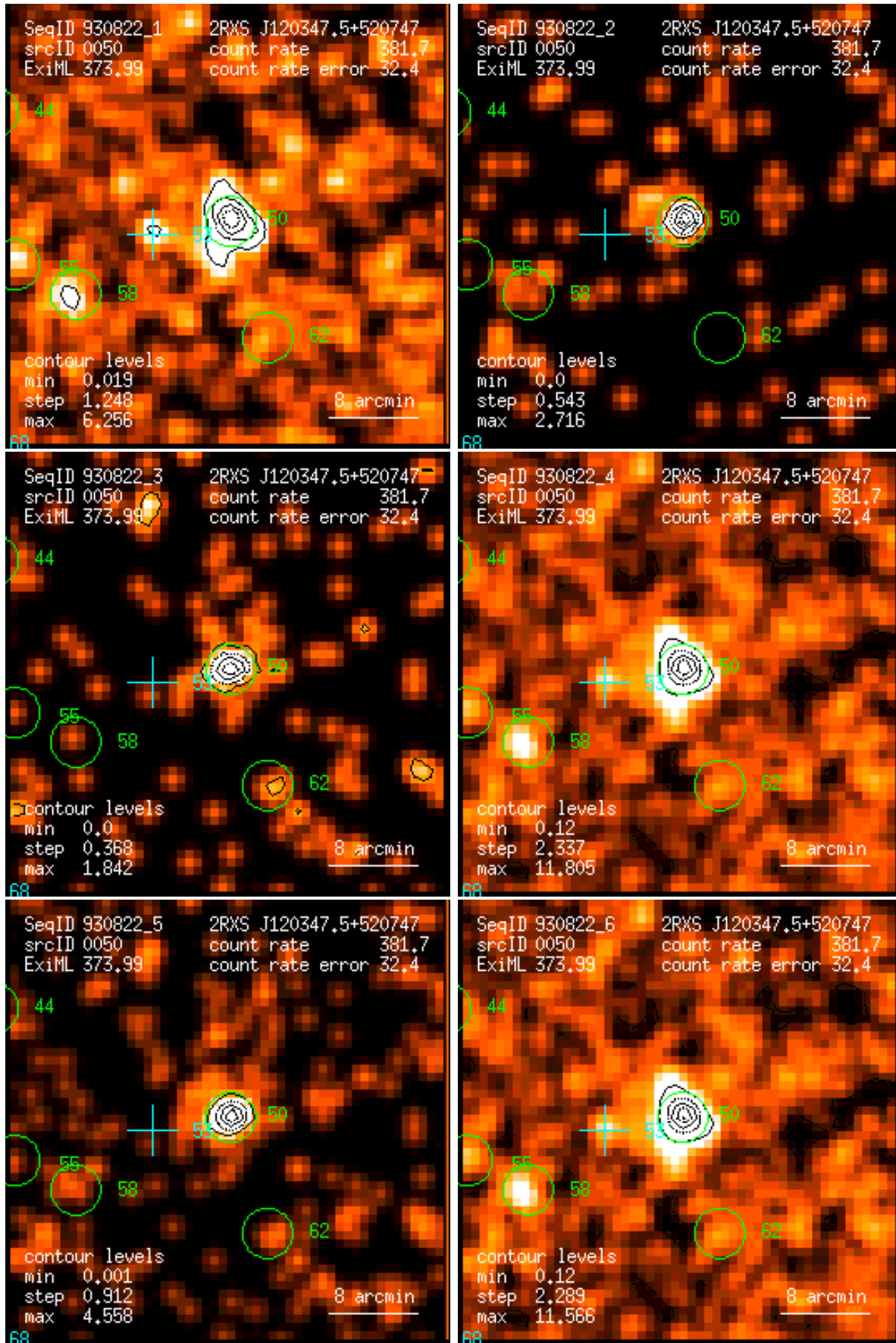
Figure 50: RASS 930822: detection 0050: band rate images, Gaussian filter: (1) PSPC channels 11 – 41, (2) 52 – 90, (3) 91 – 201, (4) 11 – 235, (5) 52 – 201, (6) 11 – 201. Broad band rates in counts/ks. Band rate contour levels in counts/ks/arcmin 2 .
