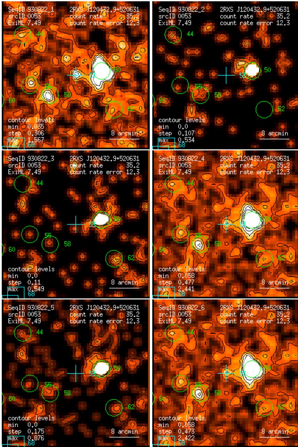
Figure 53: RASS 930822: detection 0053: band rate images, Gaussian filter: (1) PSPC channels 11 – 41, (2) 52 – 90, (3) 91 – 201, (4) 11 – 235, (5) 52 – 201, (6) 11 – 201. Broad band rates in counts/ks. Band rate contour levels in counts/ks/arcmin 2 .
