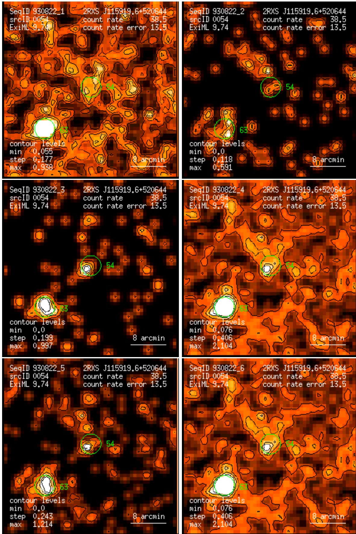
Figure 54: RASS 930822: detection 0054: band rate images, Gaussian filter: (1) PSPC channels 11 – 41, (2) 52 – 90, (3) 91 – 201, (4) 11 – 235, (5) 52 – 201, (6) 11 – 201. Broad band rates in counts/ks. Band rate contour levels in counts/ks/arcmin 2 .
