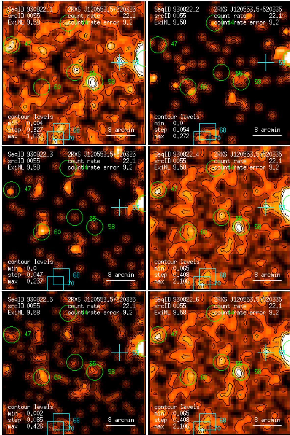
Figure 55: RASS 930822: detection 0055: band rate images, Gaussian filter: (1) PSPC channels 11 – 41, (2) 52 – 90, (3) 91 – 201, (4) 11 – 235, (5) 52 – 201, (6) 11 – 201. Broad band rates in counts/ks. Band rate contour levels in counts/ks/arcmin 2 .
