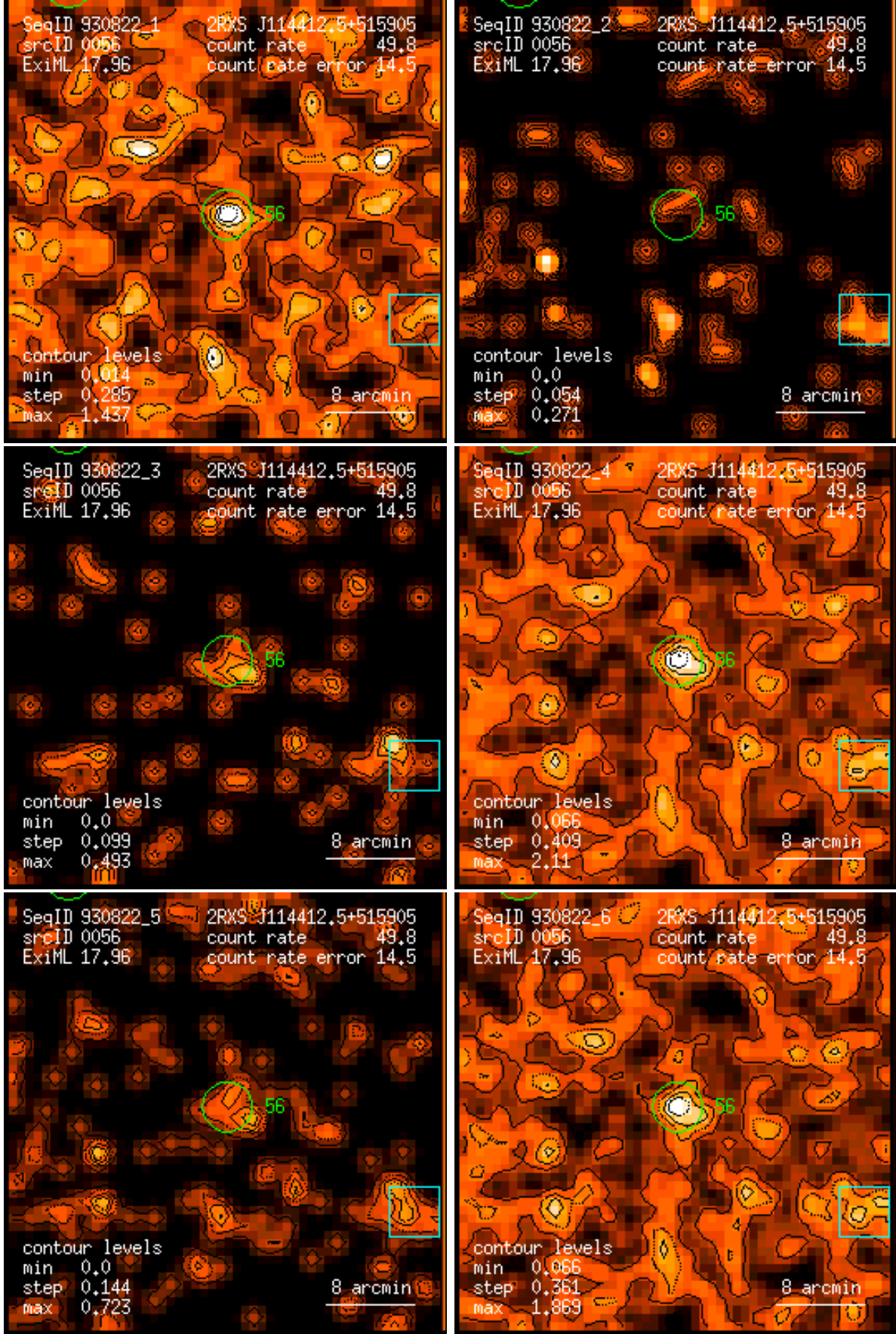
Figure 56: RASS 930822: detection 0056: band rate images, Gaussian filter: (1) PSPC channels 11 – 41, (2) 52 – 90, (3) 91 – 201, (4) 11 – 235, (5) 52 – 201, (6) 11 – 201. Broad band rates in counts/ks. Band rate contour levels in counts/ks/arcmin 2 .
