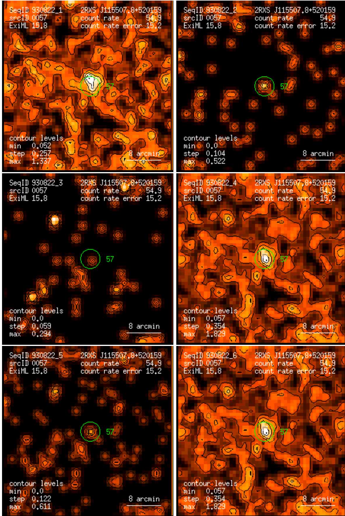
Figure 57: RASS 930822: detection 0057: band rate images, Gaussian filter: (1) PSPC channels 11 – 41, (2) 52 – 90, (3) 91 – 201, (4) 11 – 235, (5) 52 – 201, (6) 11 – 201. Broad band rates in counts/ks. Band rate contour levels in counts/ks/arcmin 2 .
