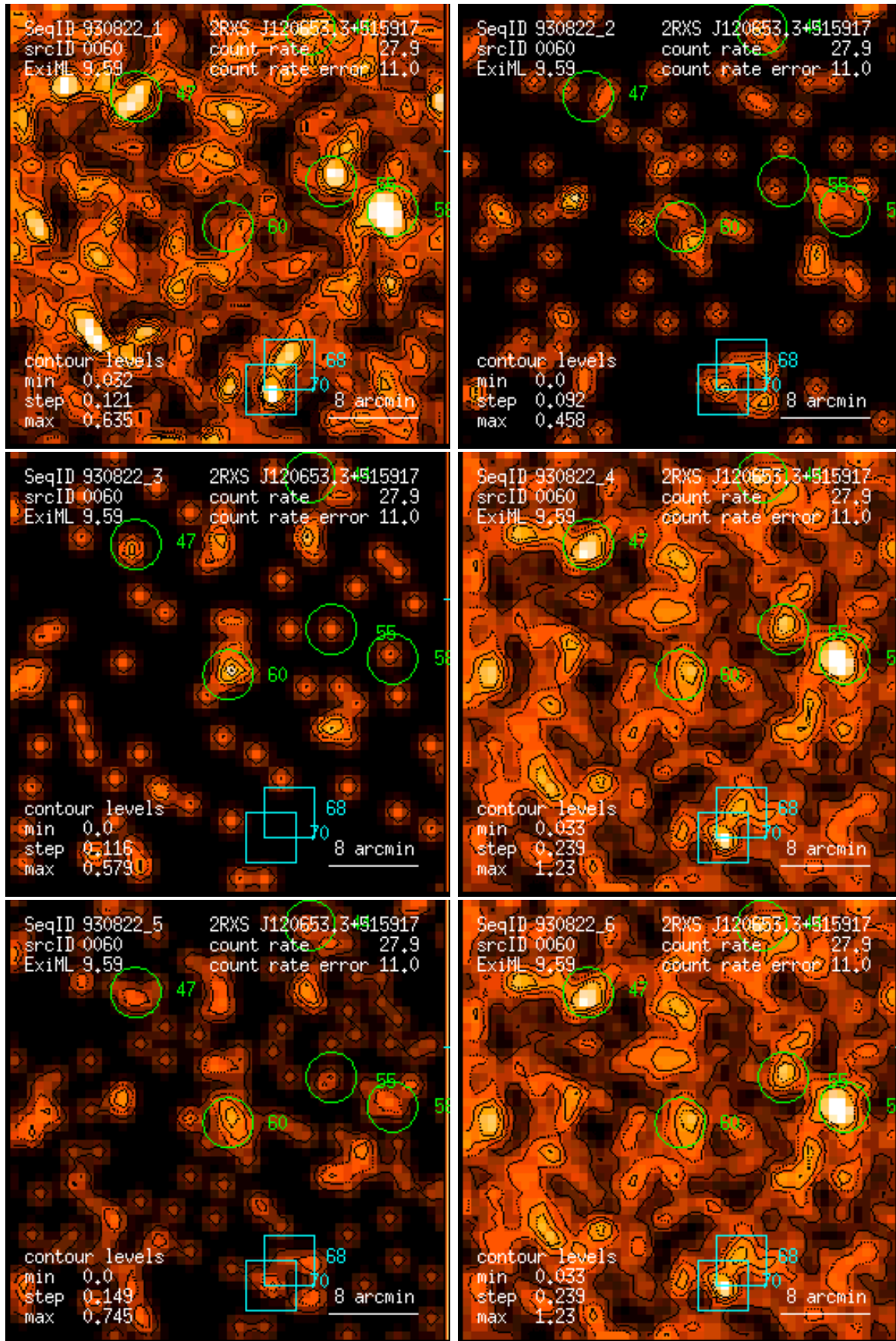
Figure 60: RASS 930822: detection 0060: band rate images, Gaussian filter: (1) PSPC channels 11 – 41, (2) 52 – 90, (3) 91 – 201, (4) 11 – 235, (5) 52 – 201, (6) 11 – 201. Broad band rates in counts/ks. Band rate contour levels in counts/ks/arcmin 2 .
