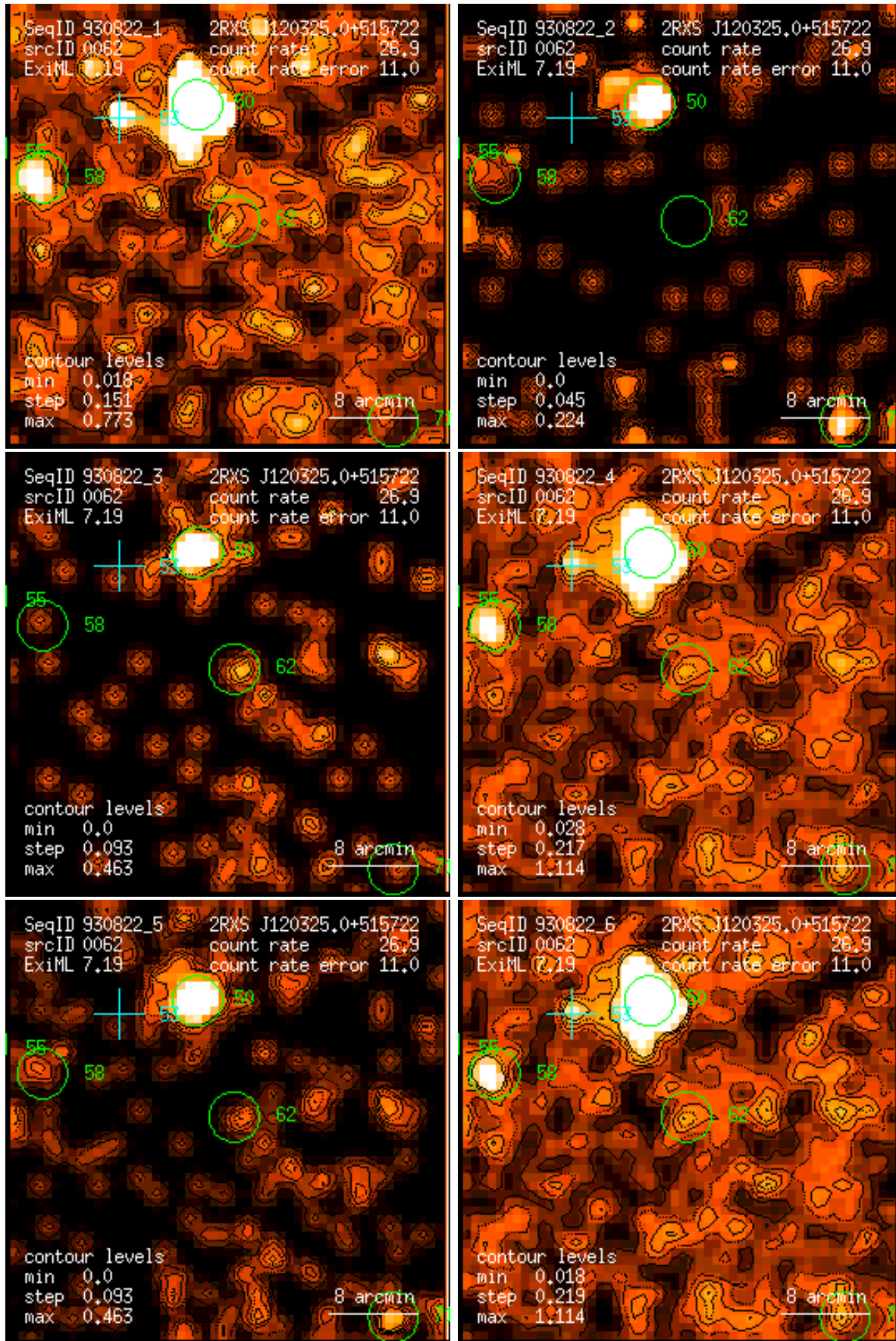
Figure 62: RASS 930822: detection 0062: band rate images, Gaussian filter: (1) PSPC channels 11 – 41, (2) 52 – 90, (3) 91 – 201, (4) 11 – 235, (5) 52 – 201, (6) 11 – 201. Broad band rates in counts/ks. Band rate contour levels in counts/ks/arcmin 2 .
