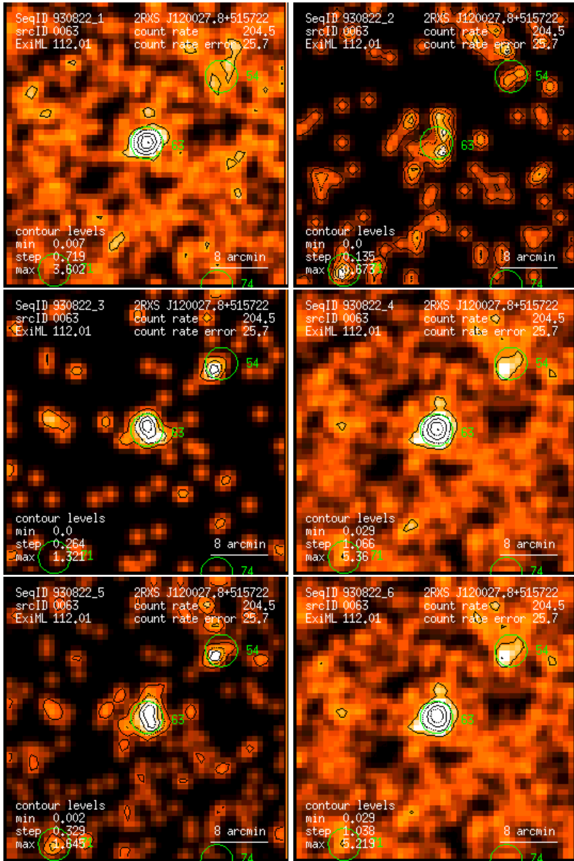
Figure 63: RASS 930822: detection 0063: band rate images, Gaussian filter: (1) PSPC channels 11 – 41, (2) 52 – 90, (3) 91 – 201, (4) 11 – 235, (5) 52 – 201, (6) 11 – 201. Broad band rates in counts/ks. Band rate contour levels in counts/ks/arcmin 2 .
