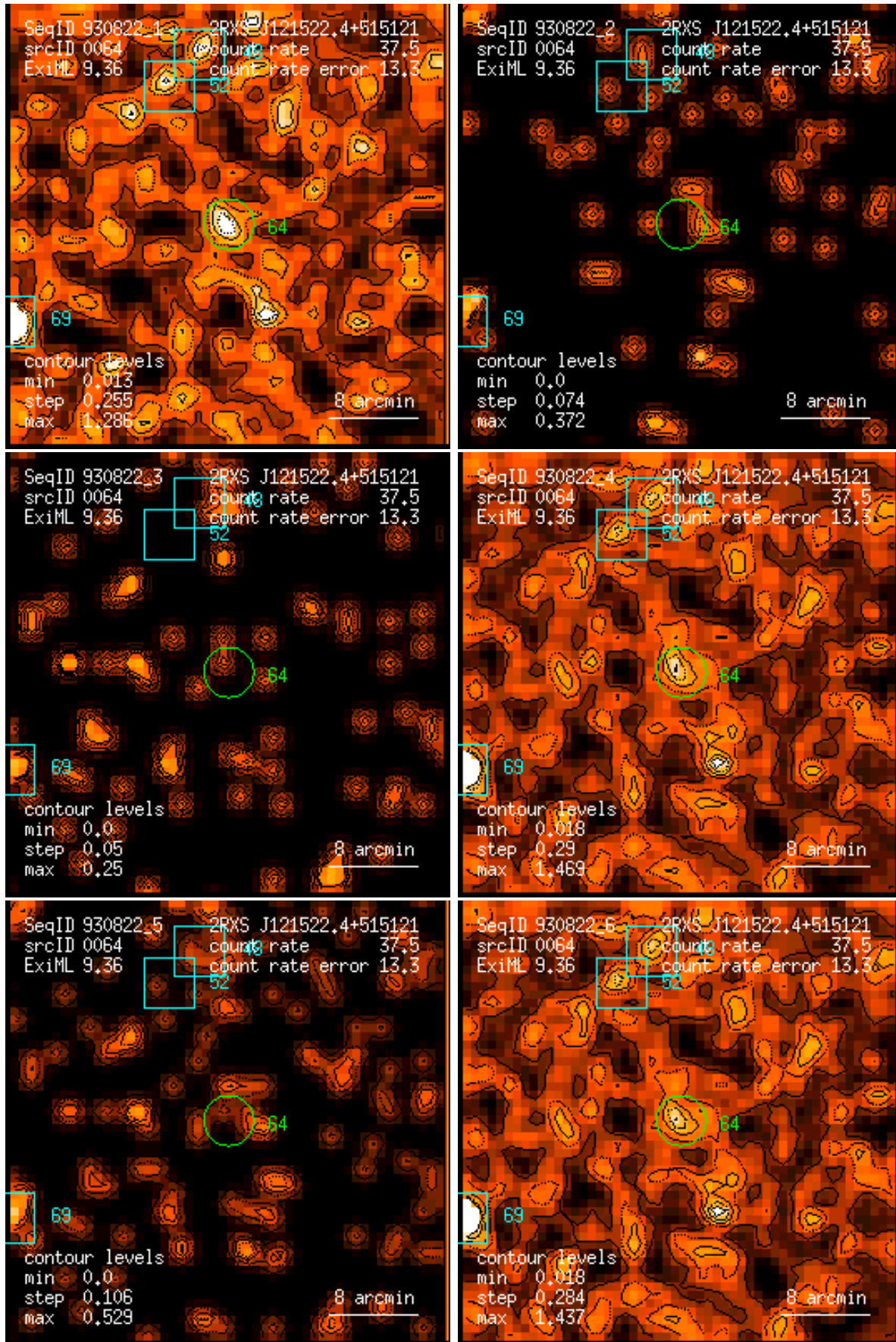
Figure 64: RASS 930822: detection 0064: band rate images, Gaussian filter: (1) PSPC channels 11 – 41, (2) 52 – 90, (3) 91 – 201, (4) 11 – 235, (5) 52 – 201, (6) 11 – 201. Broad band rates in counts/ks. Band rate contour levels in counts/ks/arcmin 2 .
