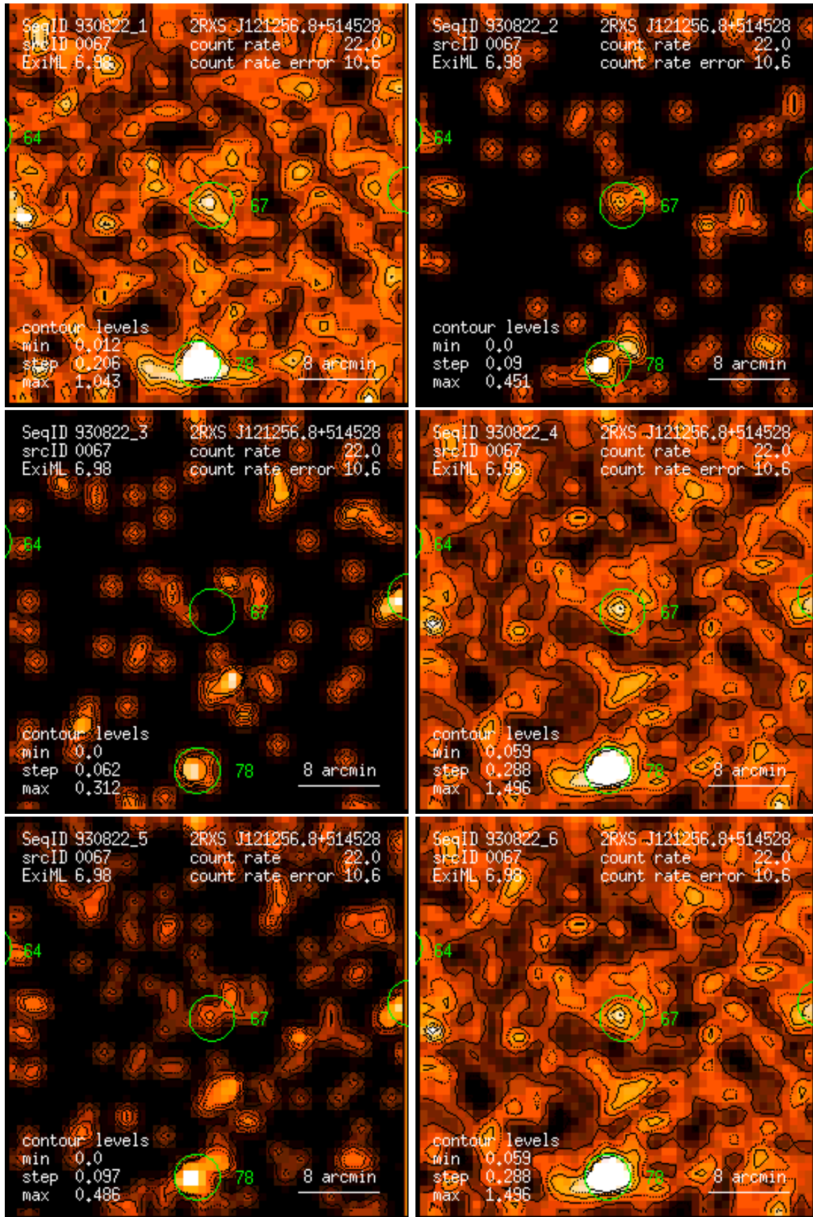
Figure 67: RASS 930822: detection 0067: band rate images, Gaussian filter: (1) PSPC channels 11 – 41, (2) 52 – 90, (3) 91 – 201, (4) 11 – 235, (5) 52 – 201, (6) 11 – 201. Broad band rates in counts/ks. Band rate contour levels in counts/ks/arcmin 2 .
