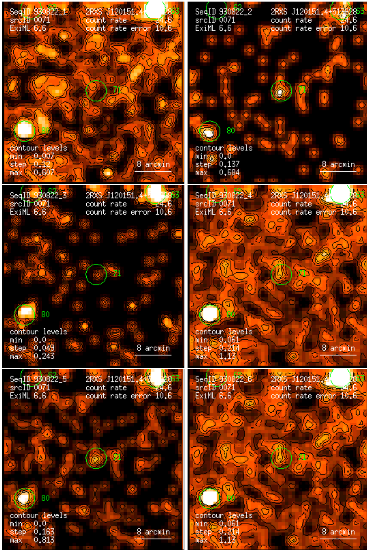
Figure 71: RASS 930822: detection 0071: band rate images, Gaussian filter: (1) PSPC channels 11 – 41, (2) 52 – 90, (3) 91 – 201, (4) 11 – 235, (5) 52 – 201, (6) 11 – 201. Broad band rates in counts/ks. Band rate contour levels in counts/ks/arcmin 2 .
