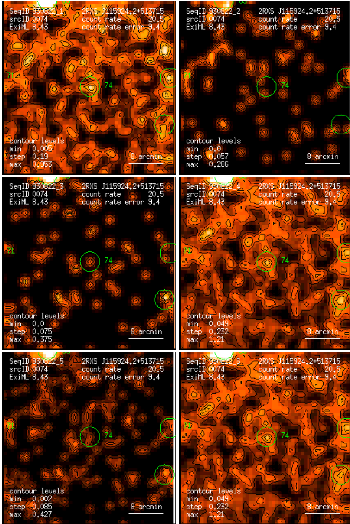
Figure 74: RASS 930822: detection 0074: band rate images, Gaussian filter: (1) PSPC channels 11 – 41, (2) 52 – 90, (3) 91 – 201, (4) 11 – 235, (5) 52 – 201, (6) 11 – 201. Broad band rates in counts/ks. Band rate contour levels in counts/ks/arcmin 2 .
